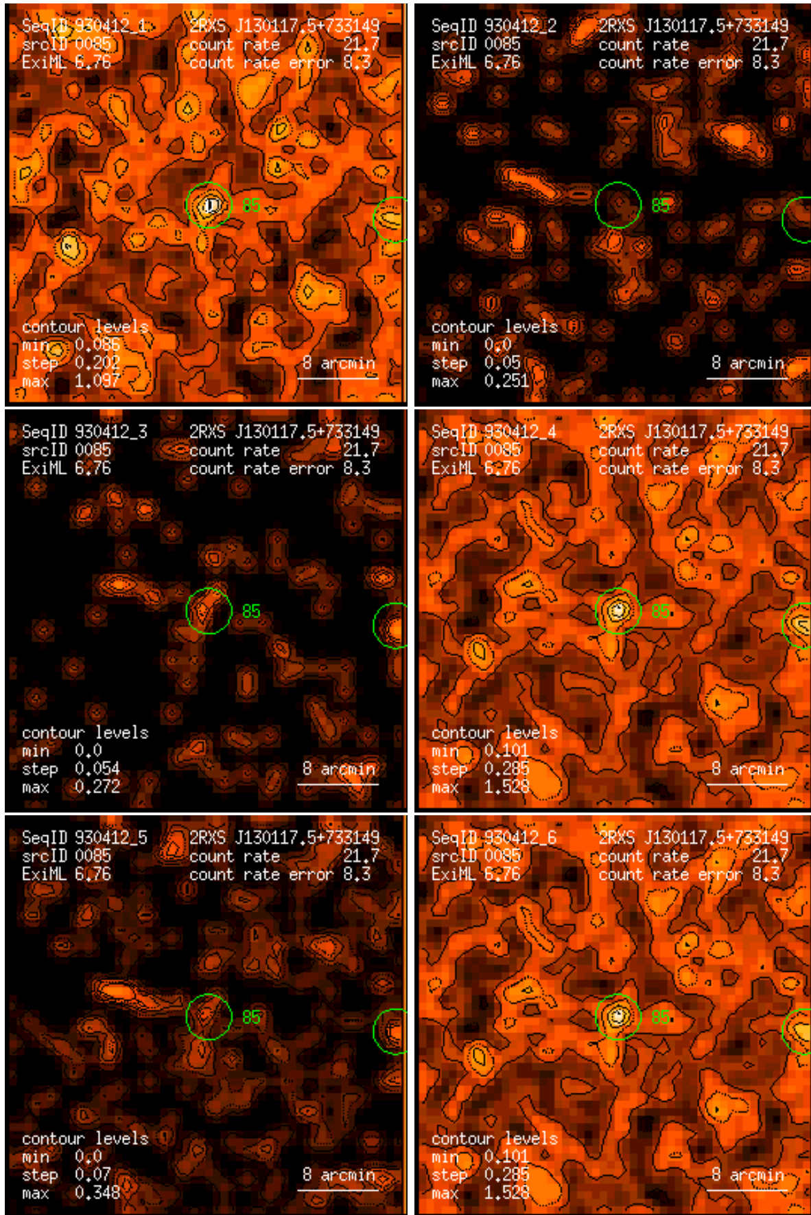
Figure 85: RASS 930412: detection 0085: band rate images, Gaussian filter: (1) PSPC channels 11 – 41, (2) 52 – 90, (3) 91 – 201, (4) 11 – 235, (5) 52 – 201, (6) 11 – 201. Broad band rates in counts/ks. Band rate contour levels in counts/ks/arcmin 2 .
