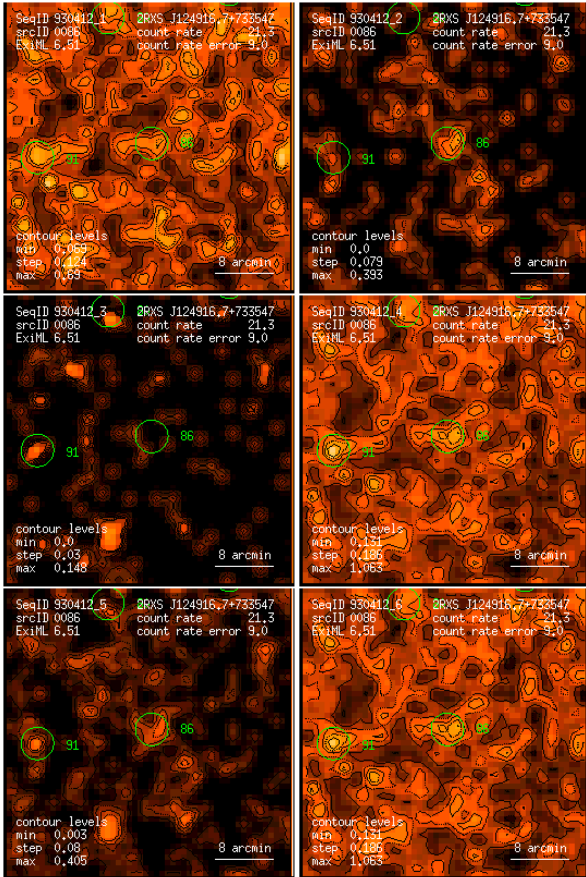
Figure 86: RASS 930412: detection 0086: band rate images, Gaussian filter: (1) PSPC channels 11 – 41, (2) 52 – 90, (3) 91 – 201, (4) 11 – 235, (5) 52 – 201, (6) 11 – 201. Broad band rates in counts/ks. Band rate contour levels in counts/ks/arcmin 2 .
