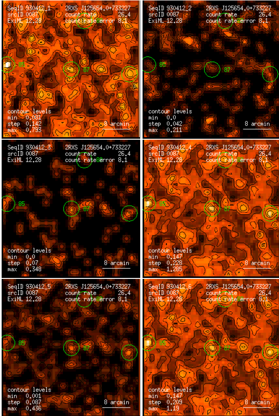
Figure 87: RASS 930412: detection 0087: band rate images, Gaussian filter: (1) PSPC channels 11 – 41, (2) 52 – 90, (3) 91 – 201, (4) 11 – 235, (5) 52 – 201, (6) 11 – 201. Broad band rates in counts/ks. Band rate contour levels in counts/ks/arcmin 2 .
