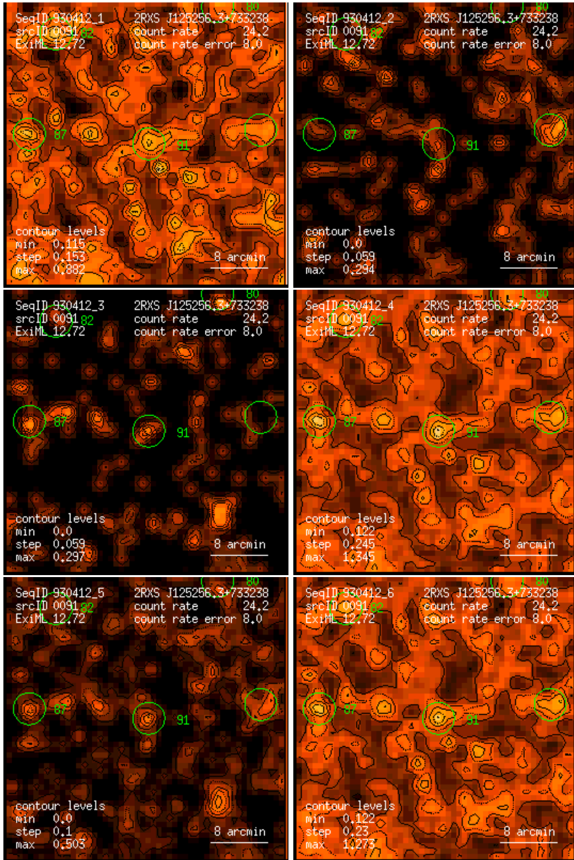
Figure 91: RASS 930412: detection 0091: band rate images, Gaussian filter: (1) PSPC channels 11 – 41, (2) 52 – 90, (3) 91 – 201, (4) 11 – 235, (5) 52 – 201, (6) 11 – 201. Broad band rates in counts/ks. Band rate contour levels in counts/ks/arcmin 2 .
