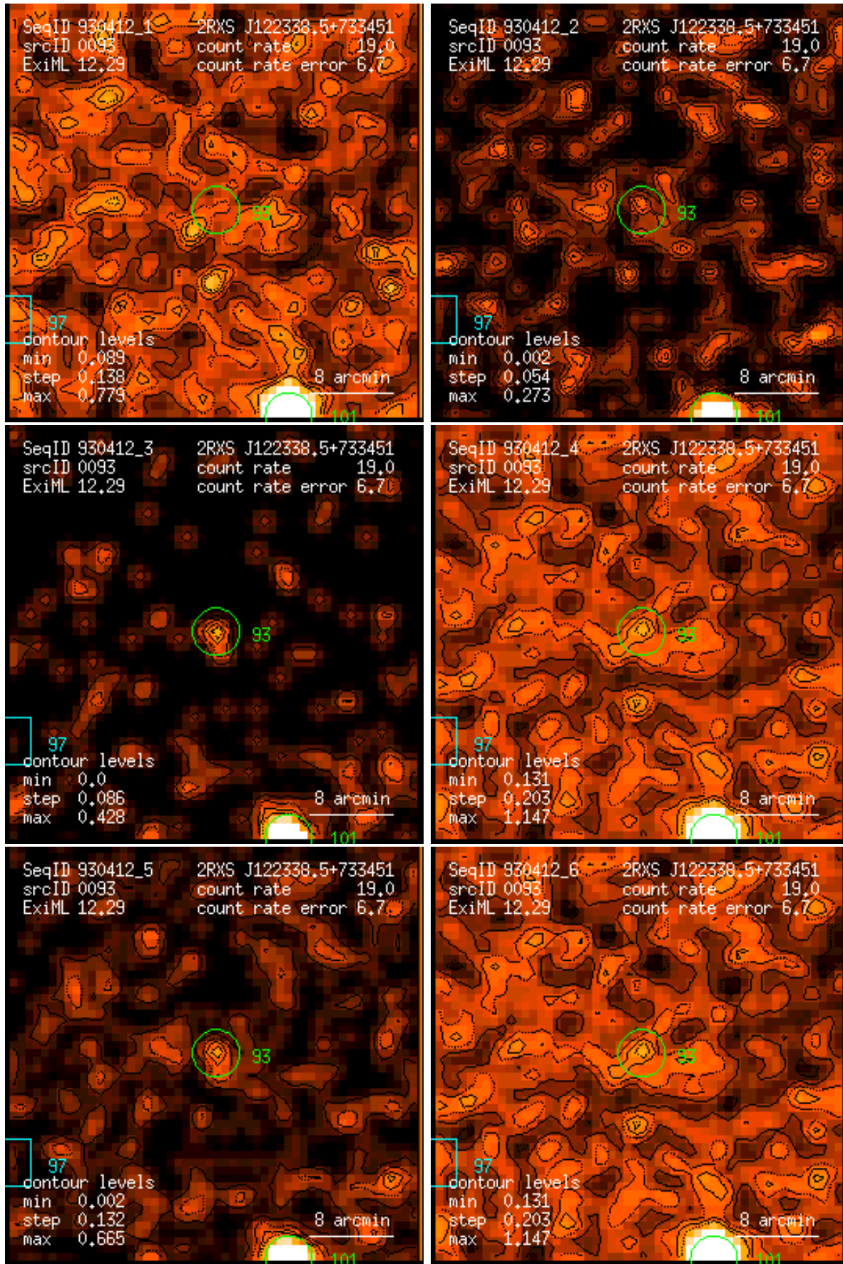
Figure 93: RASS 930412: detection 0093: band rate images, Gaussian filter: (1) PSPC channels 11 – 41, (2) 52 – 90, (3) 91 – 201, (4) 11 – 235, (5) 52 – 201, (6) 11 – 201. Broad band rates in counts/ks. Band rate contour levels in counts/ks/arcmin 2 .
