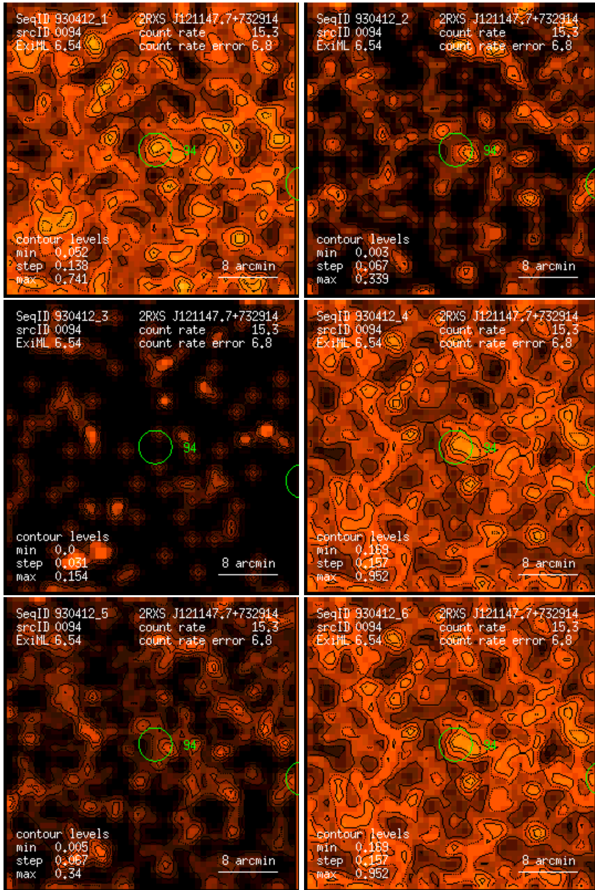
Figure 94: RASS 930412: detection 0094: band rate images, Gaussian filter: (1) PSPC channels 11 – 41, (2) 52 – 90, (3) 91 – 201, (4) 11 – 235, (5) 52 – 201, (6) 11 – 201. Broad band rates in counts/ks. Band rate contour levels in counts/ks/arcmin 2 .
