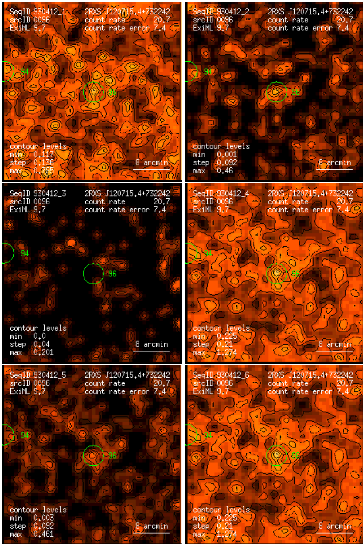
Figure 96: RASS 930412: detection 0096: band rate images, Gaussian filter: (1) PSPC channels 11 – 41, (2) 52 – 90, (3) 91 – 201, (4) 11 – 235, (5) 52 – 201, (6) 11 – 201. Broad band rates in counts/ks. Band rate contour levels in counts/ks/arcmin 2 .
