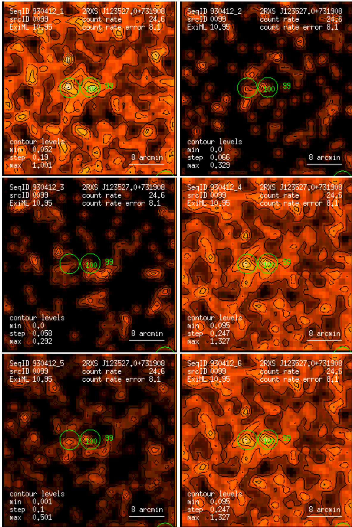
Figure 99: RASS 930412: detection 0099: band rate images, Gaussian filter: (1) PSPC channels 11 – 41, (2) 52 – 90, (3) 91 – 201, (4) 11 – 235, (5) 52 – 201, (6) 11 – 201. Broad band rates in counts/ks. Band rate contour levels in counts/ks/arcmin 2 .
