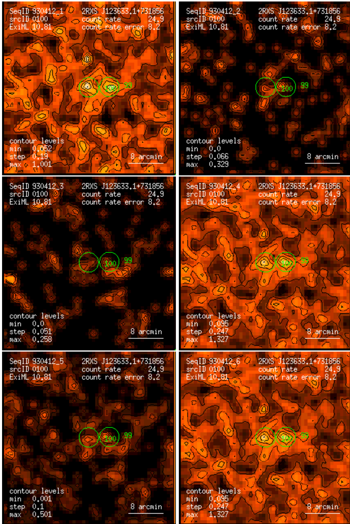
Figure 100: RASS 930412: detection 0100: band rate images, Gaussian filter: (1) PSPC channels 11 – 41, (2) 52 – 90, (3) 91 – 201, (4) 11 – 235, (5) 52 – 201, (6) 11 – 201. Broad band rates in counts/ks. Band rate contour levels in counts/ks/arcmin 2 .
