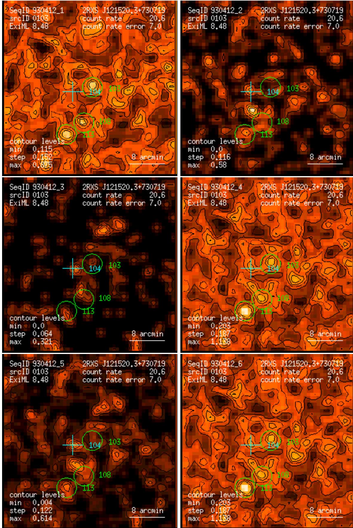
Figure 103: RASS 930412: detection 0103: band rate images, Gaussian filter: (1) PSPC channels 11 – 41, (2) 52 – 90, (3) 91 – 201, (4) 11 – 235, (5) 52 – 201, (6) 11 – 201. Broad band rates in counts/ks. Band rate contour levels in counts/ks/arcmin 2 .
