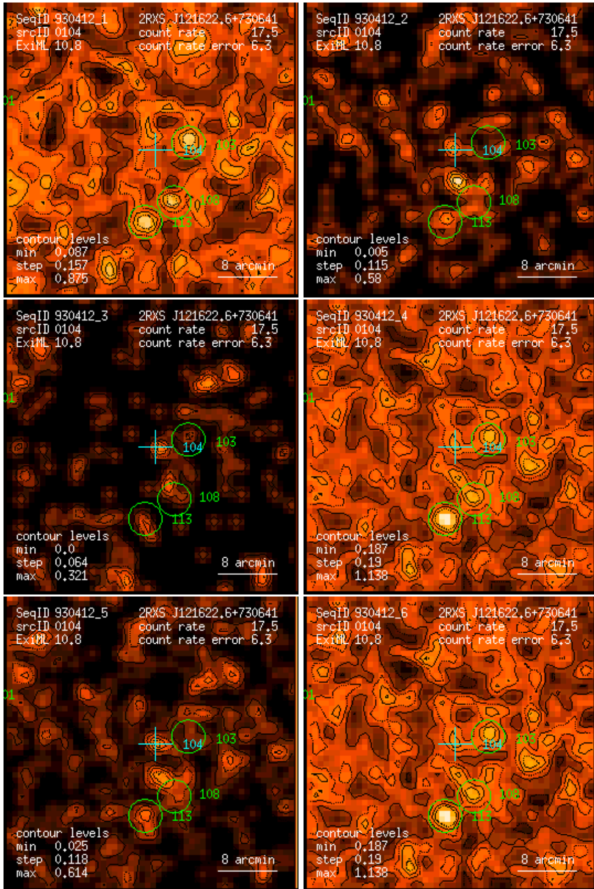
Figure 104: RASS 930412: detection 0104: band rate images, Gaussian filter: (1) PSPC channels 11 – 41, (2) 52 – 90, (3) 91 – 201, (4) 11 – 235, (5) 52 – 201, (6) 11 – 201. Broad band rates in counts/ks. Band rate contour levels in counts/ks/arcmin 2 .
