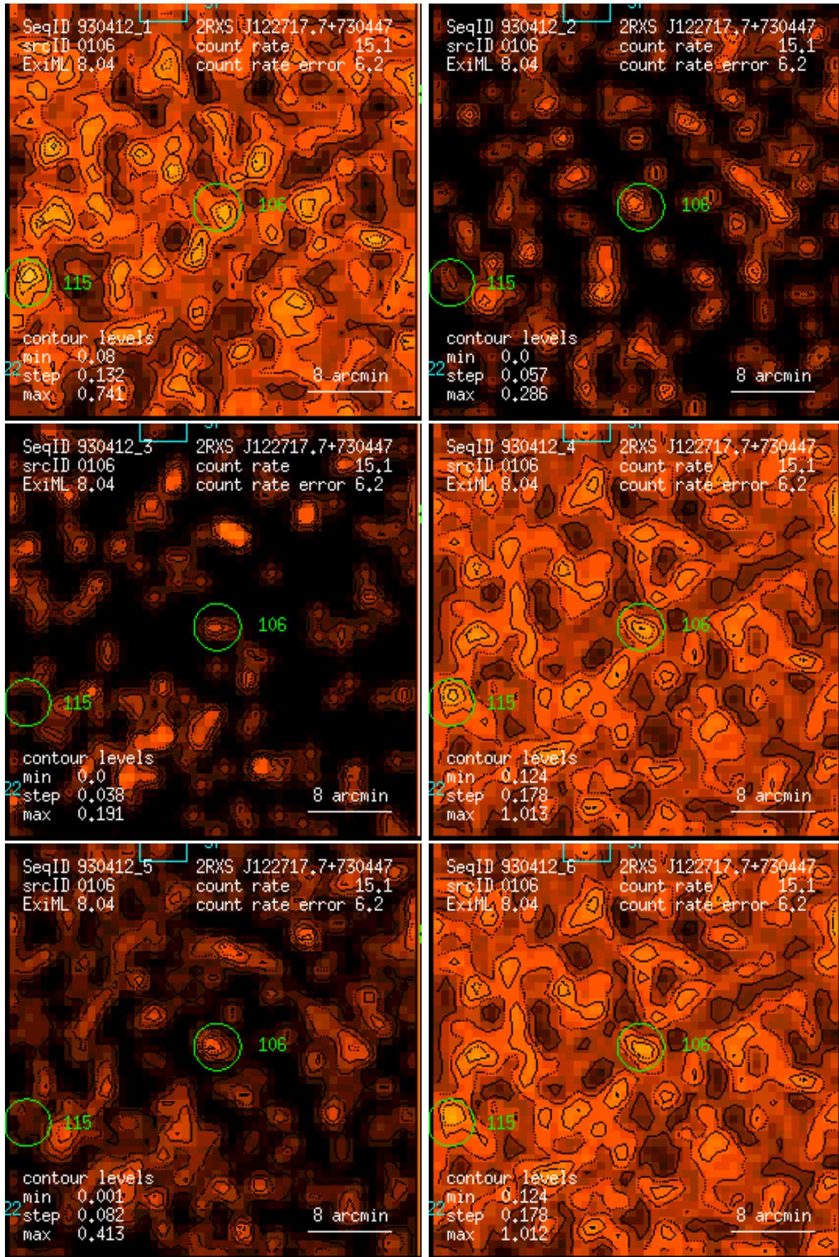
Figure 106: RASS 930412: detection 0106: band rate images, Gaussian filter: (1) PSPC channels 11 – 41, (2) 52 – 90, (3) 91 – 201, (4) 11 – 235, (5) 52 – 201, (6) 11 – 201. Broad band rates in counts/ks. Band rate contour levels in counts/ks/arcmin 2 .
