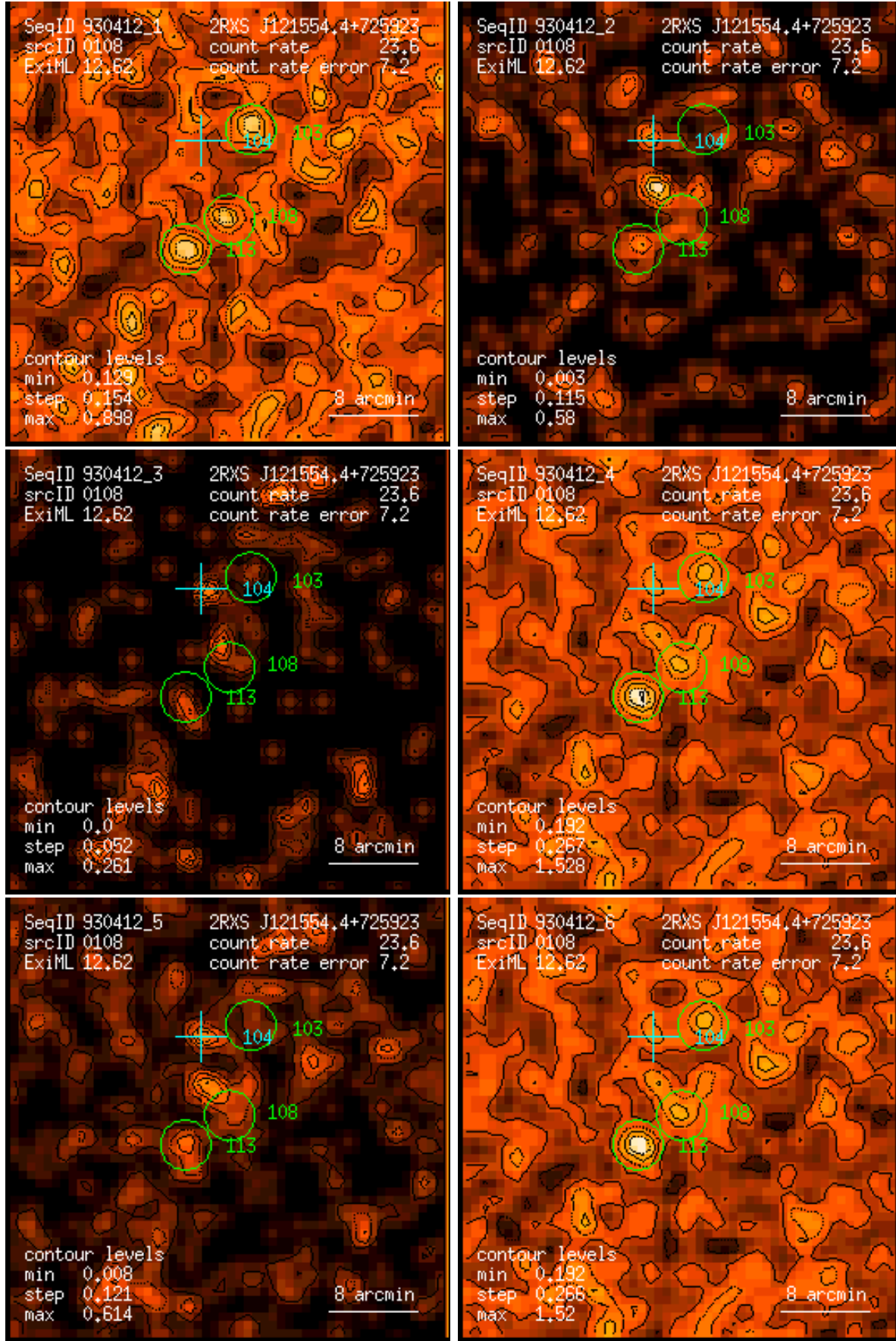
Figure 108: RASS 930412: detection 0108: band rate images, Gaussian filter: (1) PSPC channels 11 – 41, (2) 52 – 90, (3) 91 – 201, (4) 11 – 235, (5) 52 – 201, (6) 11 – 201. Broad band rates in counts/ks. Band rate contour levels in counts/ks/arcmin 2 .
