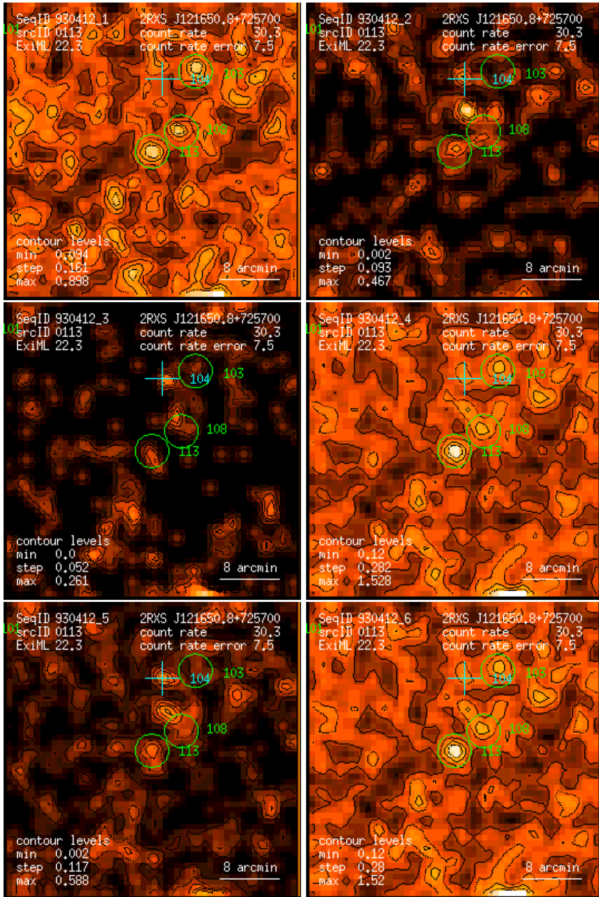
Figure 113: RASS 930412: detection 0113: band rate images, Gaussian filter: (1) PSPC channels 11 – 41, (2) 52 – 90, (3) 91 – 201, (4) 11 – 235, (5) 52 – 201, (6) 11 – 201. Broad band rates in counts/ks. Band rate contour levels in counts/ks/arcmin 2 .
