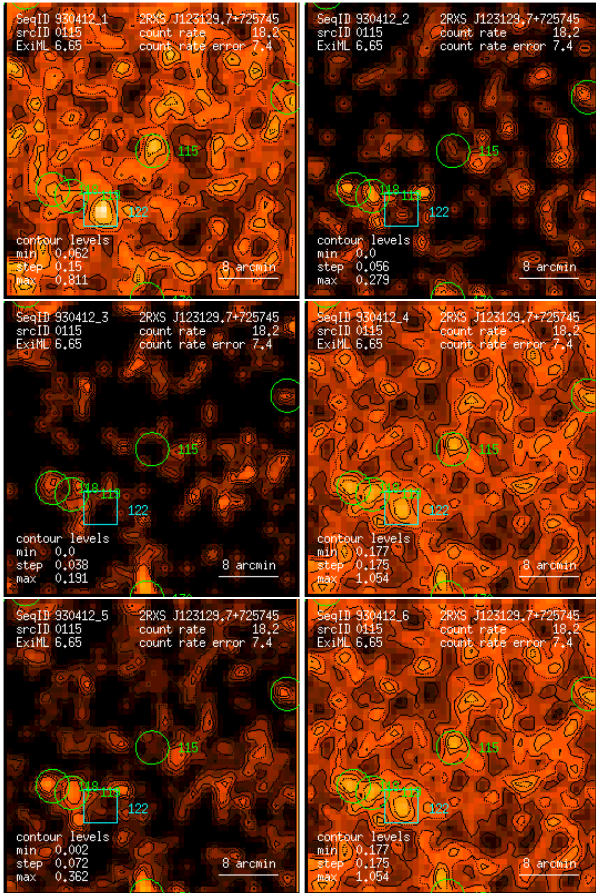
Figure 115: RASS 930412: detection 0115: band rate images, Gaussian filter: (1) PSPC channels 11 – 41, (2) 52 – 90, (3) 91 – 201, (4) 11 – 235, (5) 52 – 201, (6) 11 – 201. Broad band rates in counts/ks. Band rate contour levels in counts/ks/arcmin 2 .
