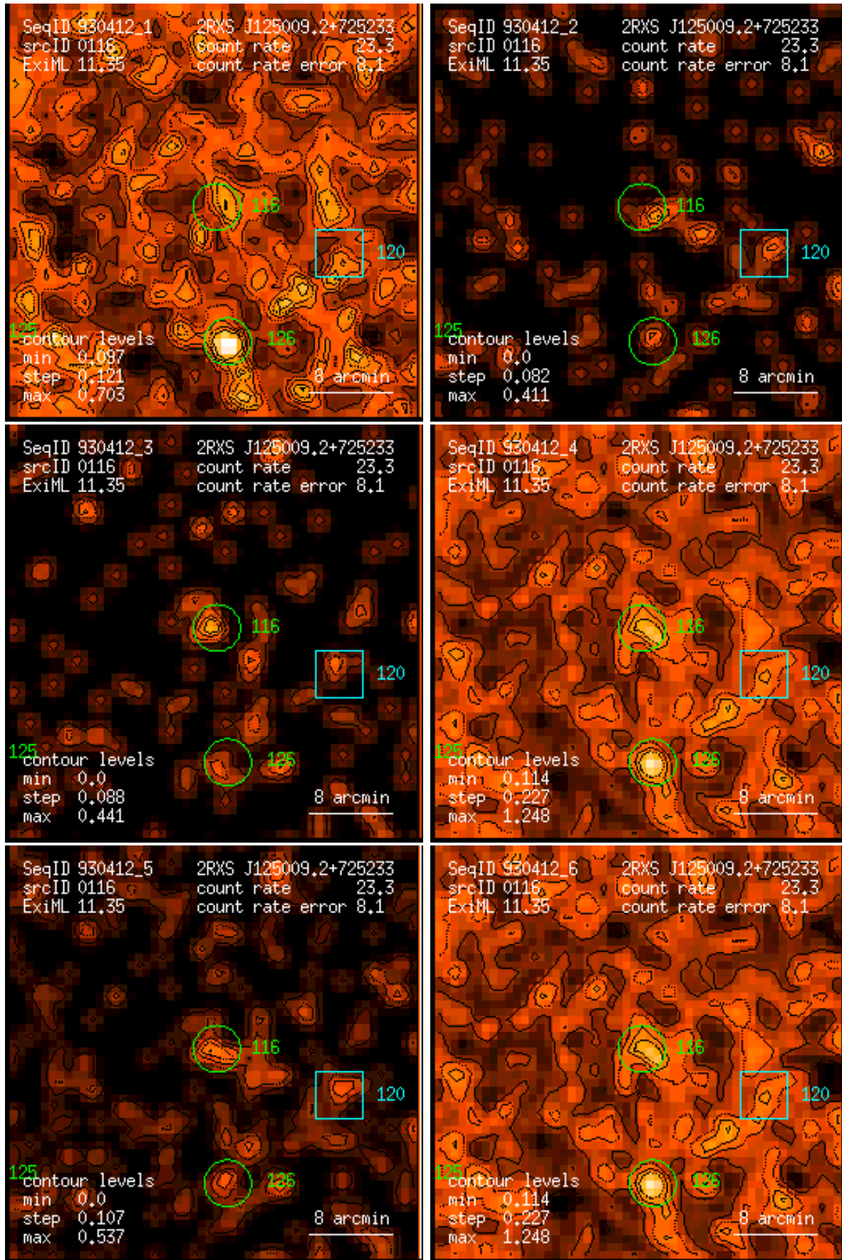
Figure 116: RASS 930412: detection 0116: band rate images, Gaussian filter: (1) PSPC channels 11 – 41, (2) 52 – 90, (3) 91 – 201, (4) 11 – 235, (5) 52 – 201, (6) 11 – 201. Broad band rates in counts/ks. Band rate contour levels in counts/ks/arcmin 2 .
