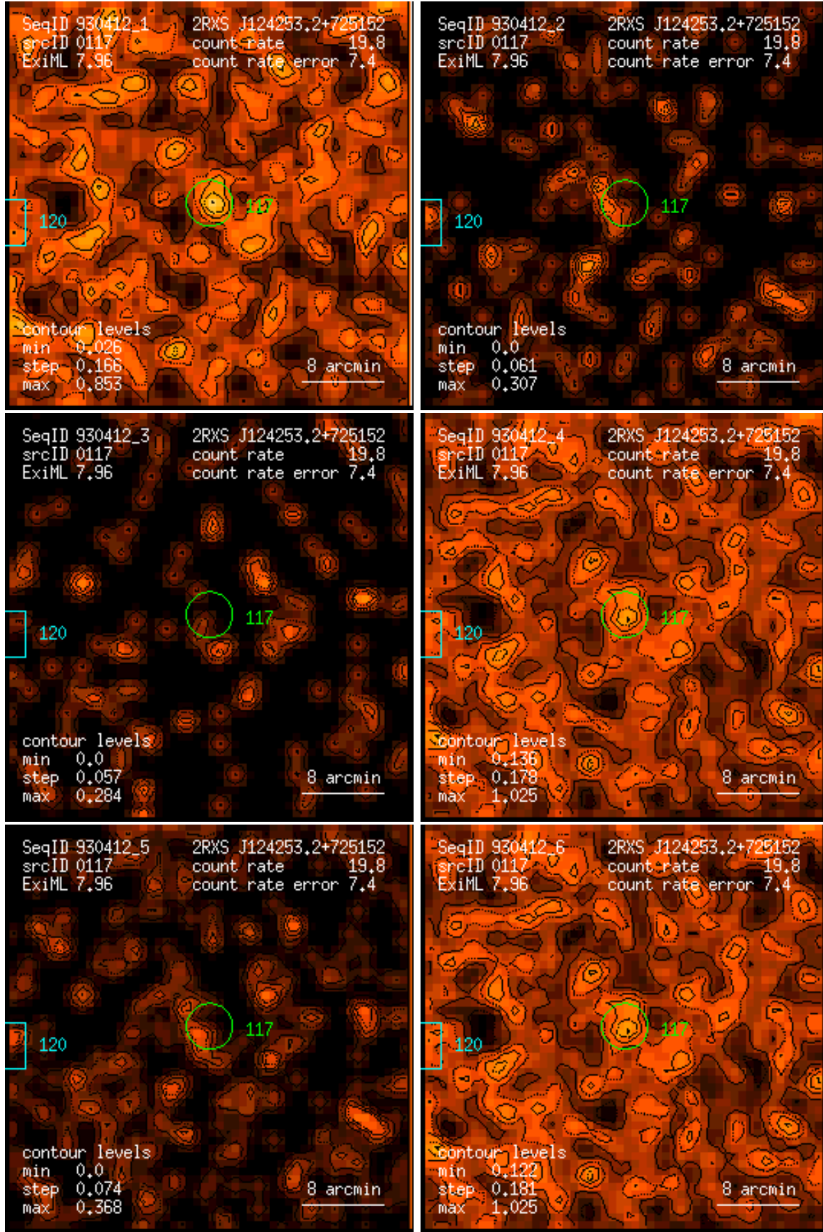
Figure 117: RASS 930412: detection 0117: band rate images, Gaussian filter: (1) PSPC channels 11 – 41, (2) 52 – 90, (3) 91 – 201, (4) 11 – 235, (5) 52 – 201, (6) 11 – 201. Broad band rates in counts/ks. Band rate contour levels in counts/ks/arcmin 2 .
