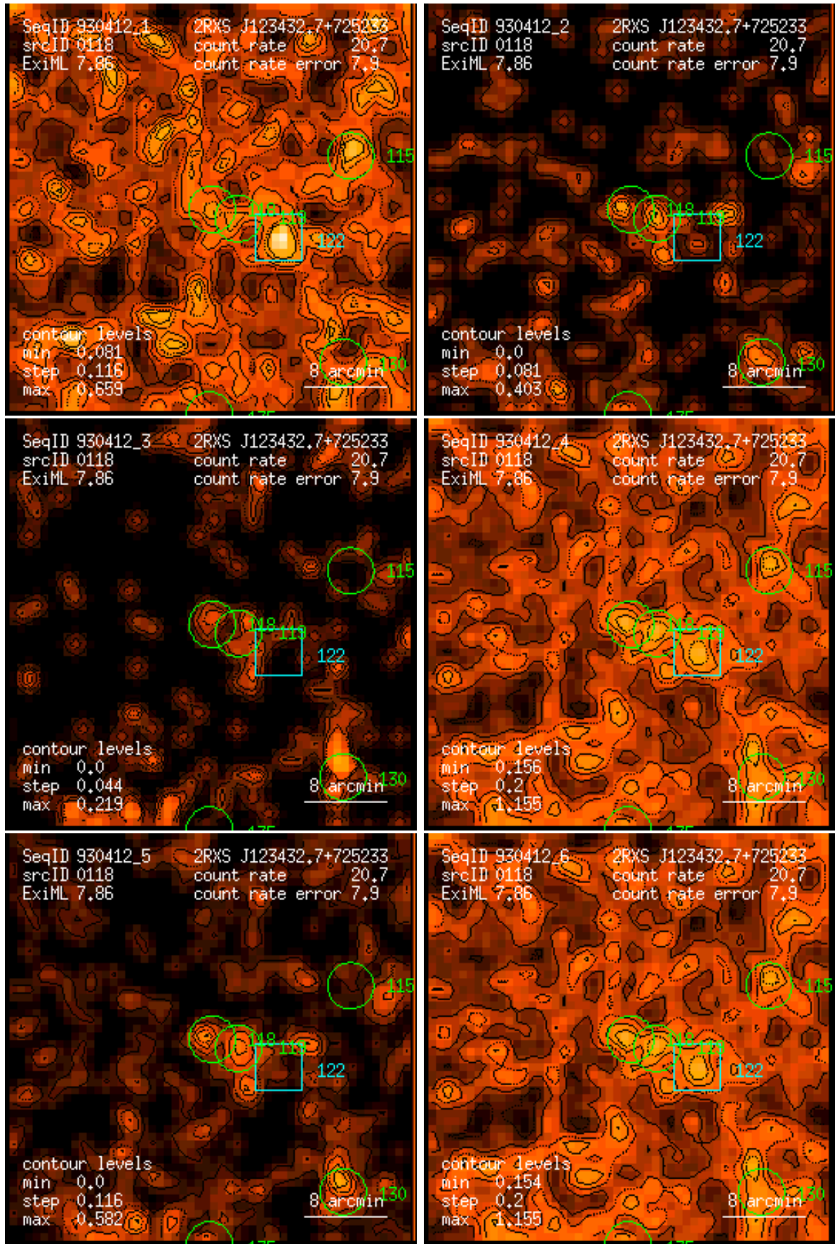
Figure 118: RASS 930412: detection 0118: band rate images, Gaussian filter: (1) PSPC channels 11 – 41, (2) 52 – 90, (3) 91 – 201, (4) 11 – 235, (5) 52 – 201, (6) 11 – 201. Broad band rates in counts/ks. Band rate contour levels in counts/ks/arcmin 2 .
