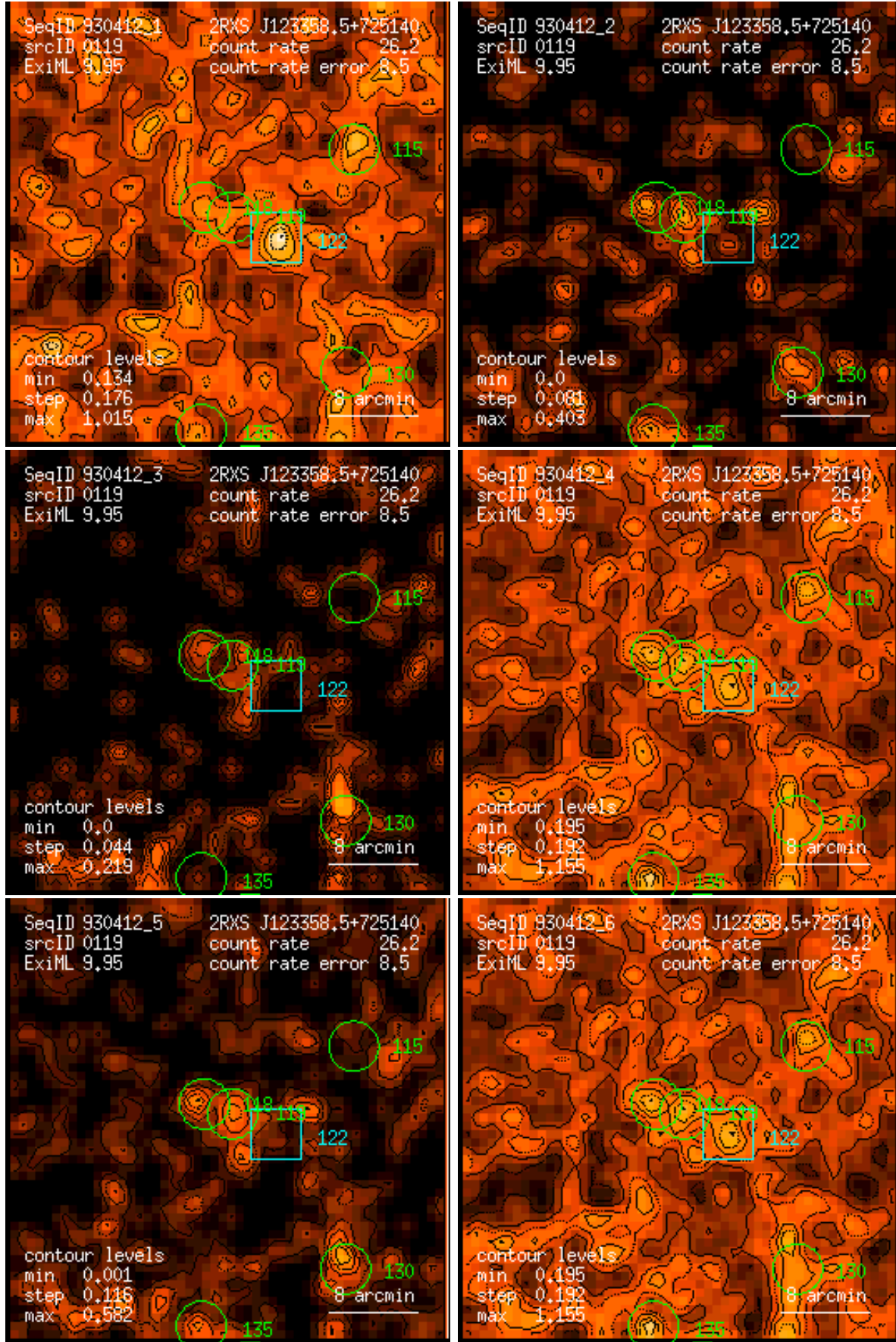
Figure 119: RASS 930412: detection 0119: band rate images, Gaussian filter: (1) PSPC channels 11 – 41, (2) 52 – 90, (3) 91 – 201, (4) 11 – 235, (5) 52 – 201, (6) 11 – 201. Broad band rates in counts/ks. Band rate contour levels in counts/ks/arcmin 2 .
