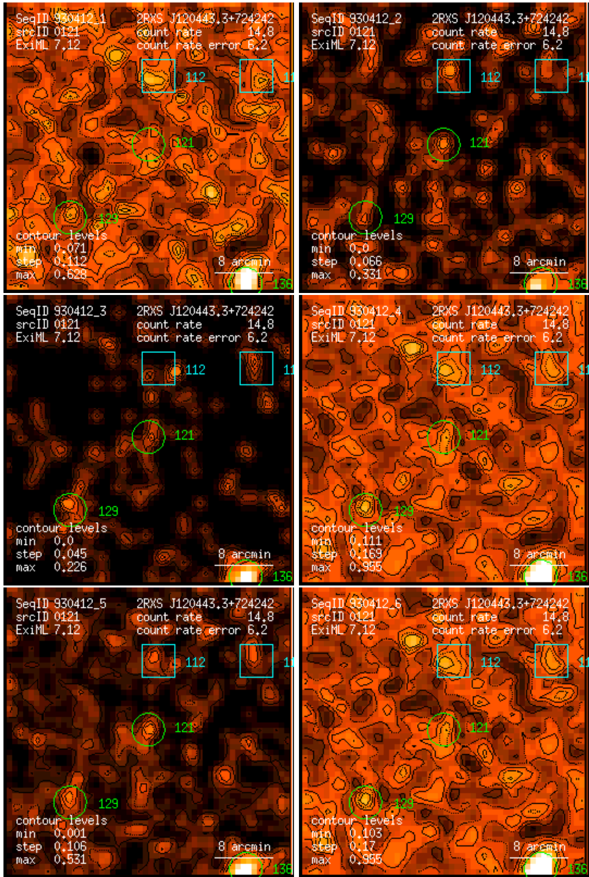
Figure 121: RASS 930412: detection 0121: band rate images, Gaussian filter: (1) PSPC channels 11 – 41, (2) 52 – 90, (3) 91 – 201, (4) 11 – 235, (5) 52 – 201, (6) 11 – 201. Broad band rates in counts/ks. Band rate contour levels in counts/ks/arcmin 2 .
