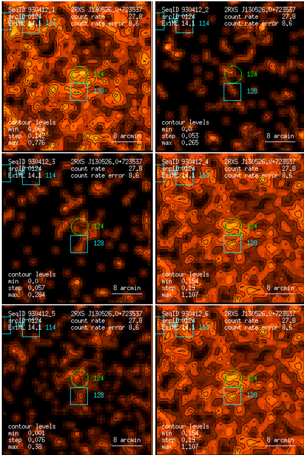
Figure 124: RASS 930412: detection 0124: band rate images, Gaussian filter: (1) PSPC channels 11 – 41, (2) 52 – 90, (3) 91 – 201, (4) 11 – 235, (5) 52 – 201, (6) 11 – 201. Broad band rates in counts/ks. Band rate contour levels in counts/ks/arcmin 2 .
