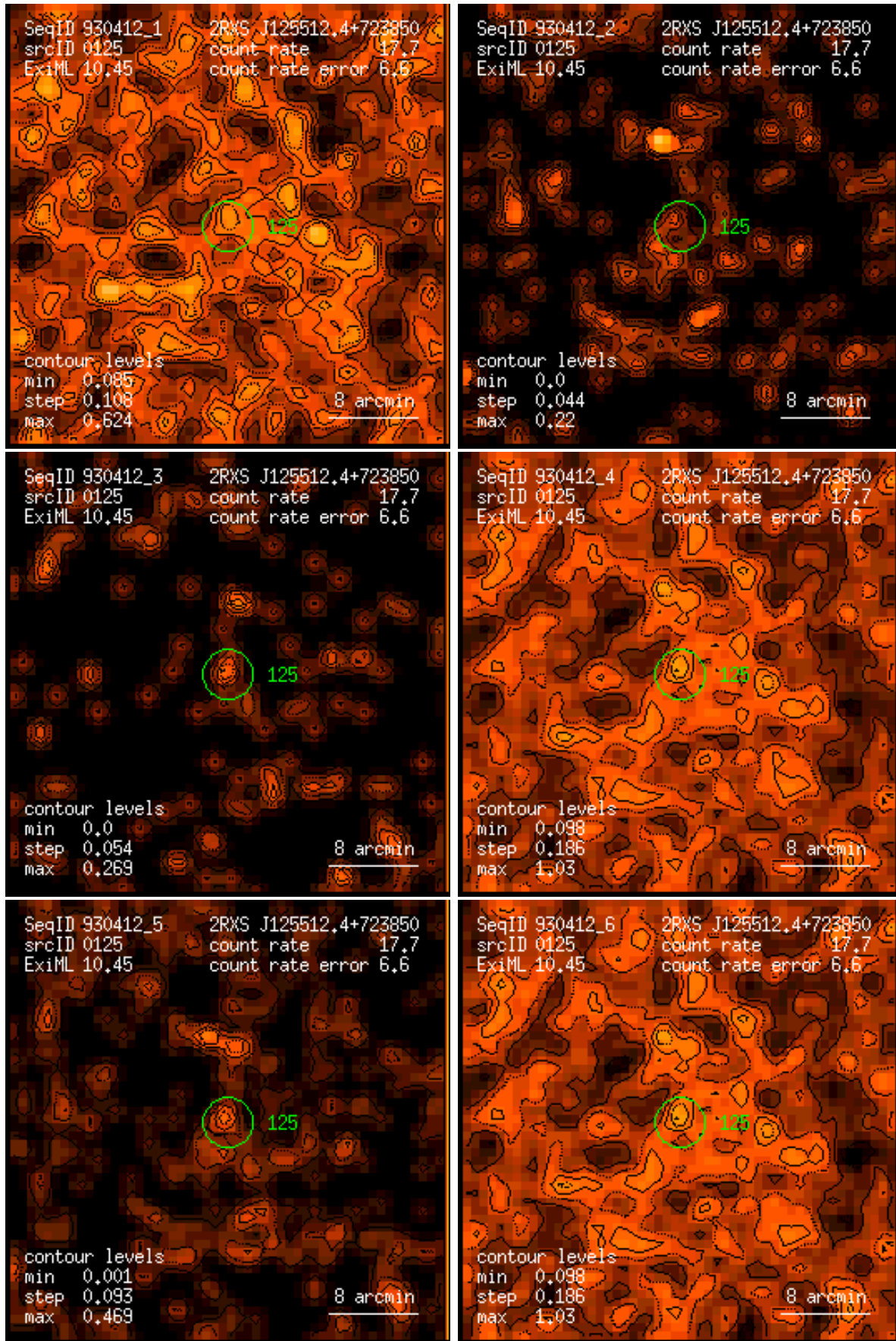
Figure 125: RASS 930412: detection 0125: band rate images, Gaussian filter: (1) PSPC channels 11 – 41, (2) 52 – 90, (3) 91 – 201, (4) 11 – 235, (5) 52 – 201, (6) 11 – 201. Broad band rates in counts/ks. Band rate contour levels in counts/ks/arcmin 2 .
