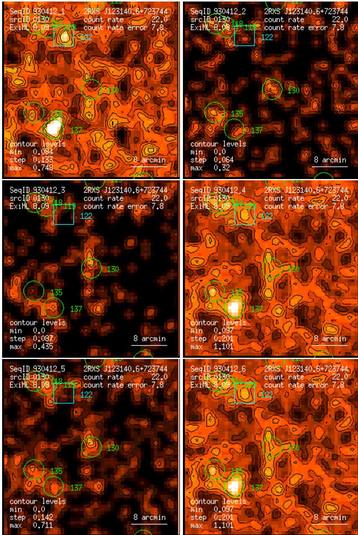
Figure 130: RASS 930412: detection 0130: band rate images, Gaussian filter: (1) PSPC channels 11 – 41, (2) 52 – 90, (3) 91 – 201, (4) 11 – 235, (5) 52 – 201, (6) 11 – 201. Broad band rates in counts/ks. Band rate contour levels in counts/ks/arcmin 2 .
