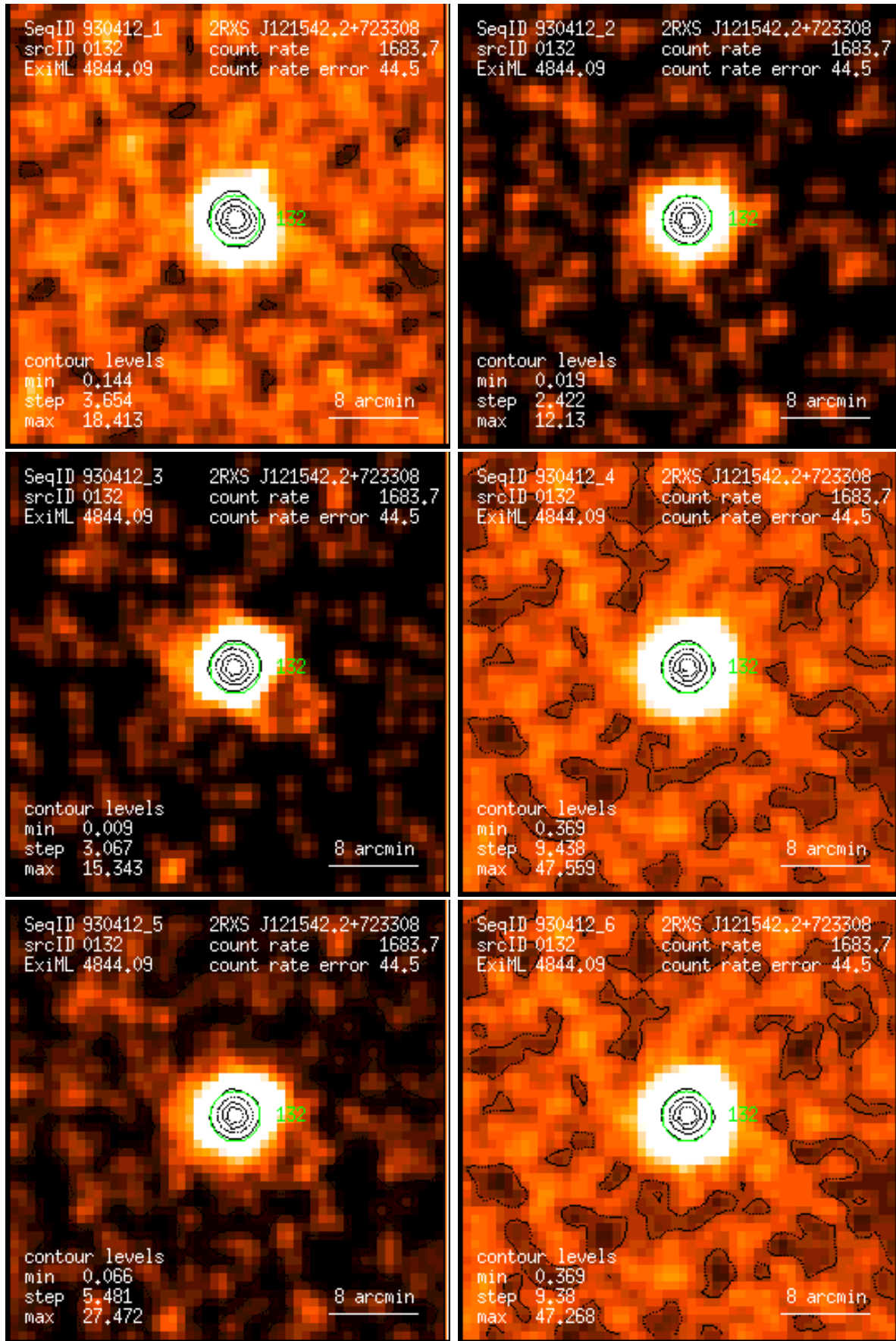
Figure 132: RASS 930412: detection 0132: band rate images, Gaussian filter: (1) PSPC channels 11 – 41, (2) 52 – 90, (3) 91 – 201, (4) 11 – 235, (5) 52 – 201, (6) 11 – 201. Broad band rates in counts/ks. Band rate contour levels in counts/ks/arcmin 2 .
