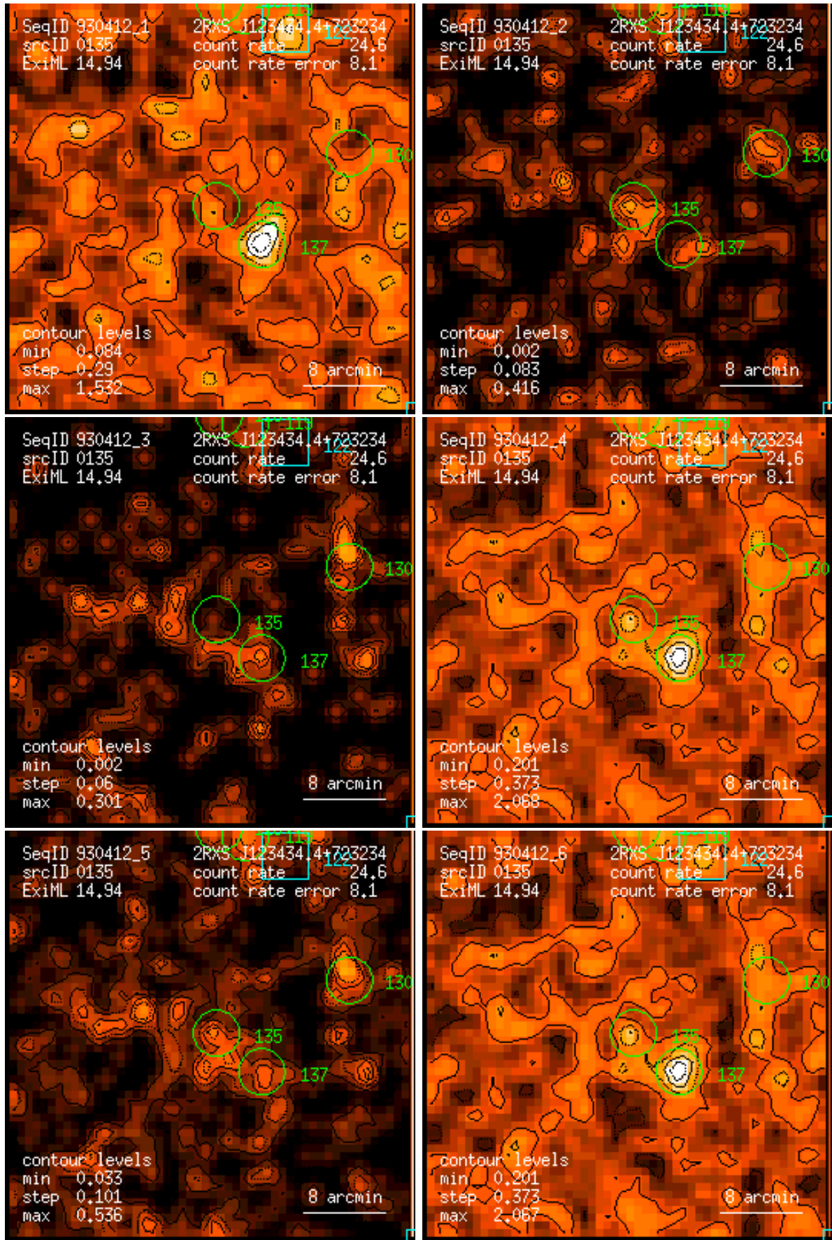
Figure 135: RASS 930412: detection 0135: band rate images, Gaussian filter: (1) PSPC channels 11 – 41, (2) 52 – 90, (3) 91 – 201, (4) 11 – 235, (5) 52 – 201, (6) 11 – 201. Broad band rates in counts/ks. Band rate contour levels in counts/ks/arcmin 2 .
