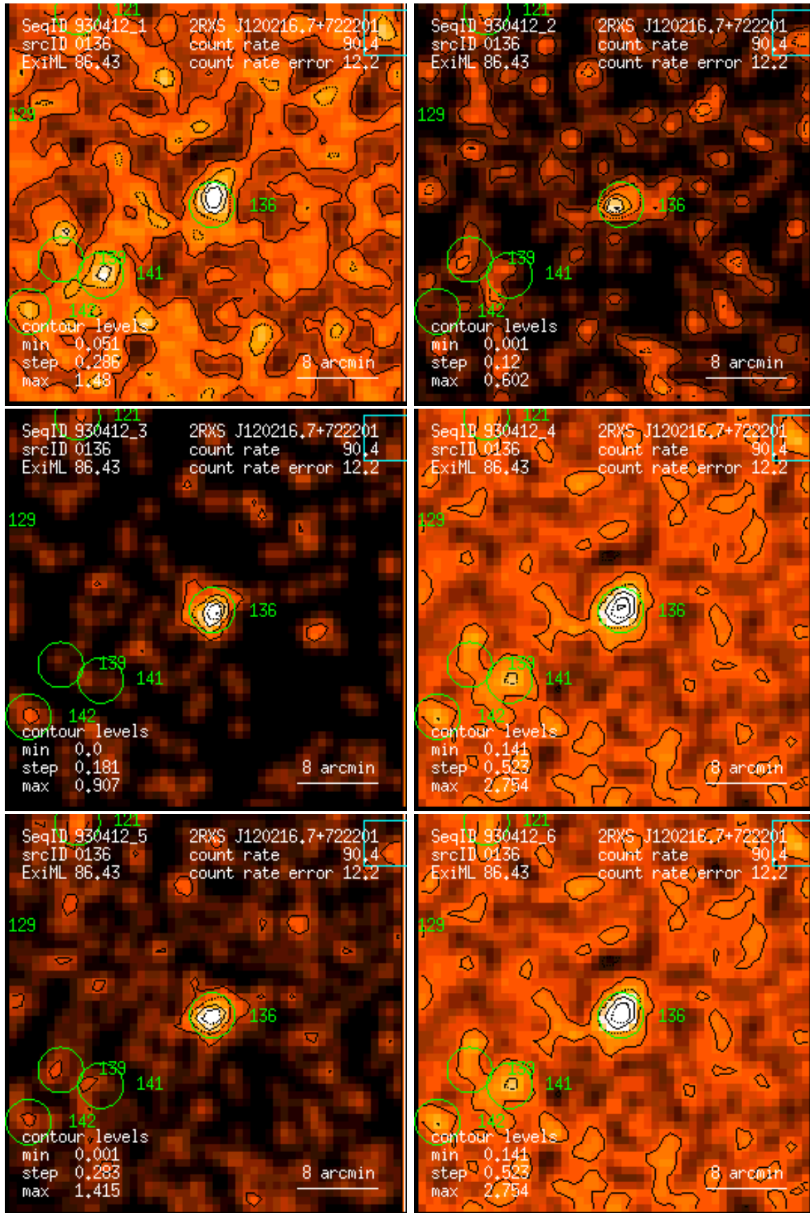
Figure 136: RASS 930412: detection 0136: band rate images, Gaussian filter: (1) PSPC channels 11 – 41, (2) 52 – 90, (3) 91 – 201, (4) 11 – 235, (5) 52 – 201, (6) 11 – 201. Broad band rates in counts/ks. Band rate contour levels in counts/ks/arcmin 2 .
