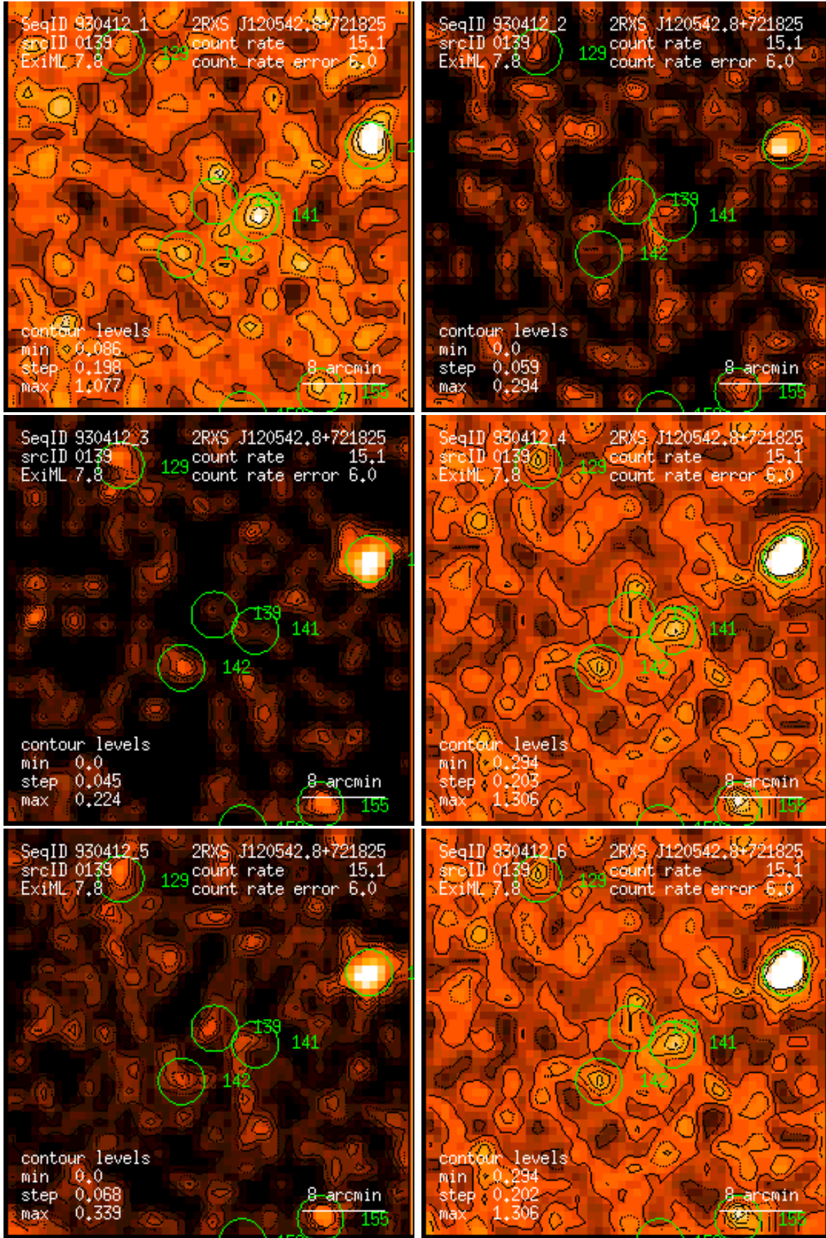
Figure 139: RASS 930412: detection 0139: band rate images, Gaussian filter: (1) PSPC channels 11 – 41, (2) 52 – 90, (3) 91 – 201, (4) 11 – 235, (5) 52 – 201, (6) 11 – 201. Broad band rates in counts/ks. Band rate contour levels in counts/ks/arcmin 2 .
