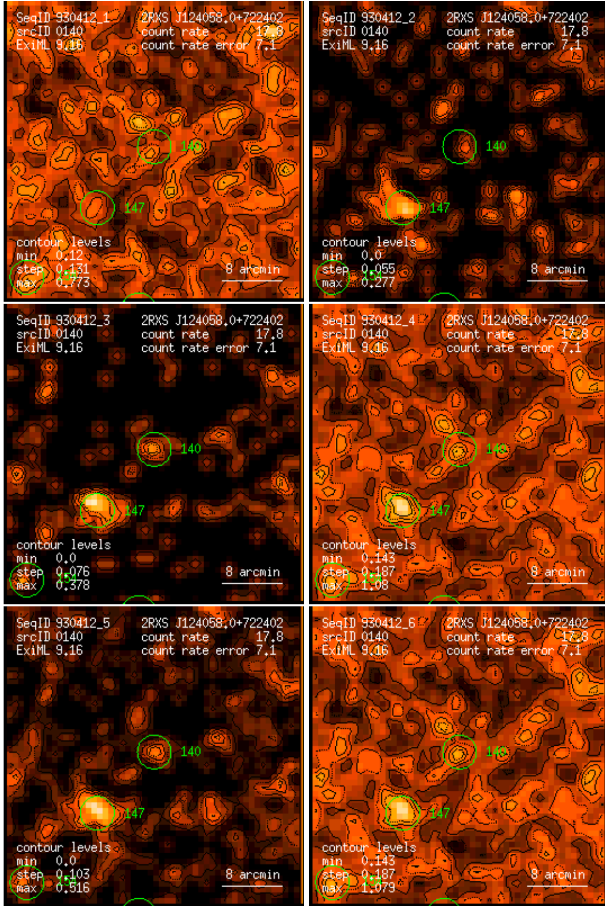
Figure 140: RASS 930412: detection 0140: band rate images, Gaussian filter: (1) PSPC channels 11 – 41, (2) 52 – 90, (3) 91 – 201, (4) 11 – 235, (5) 52 – 201, (6) 11 – 201. Broad band rates in counts/ks. Band rate contour levels in counts/ks/arcmin 2 .
