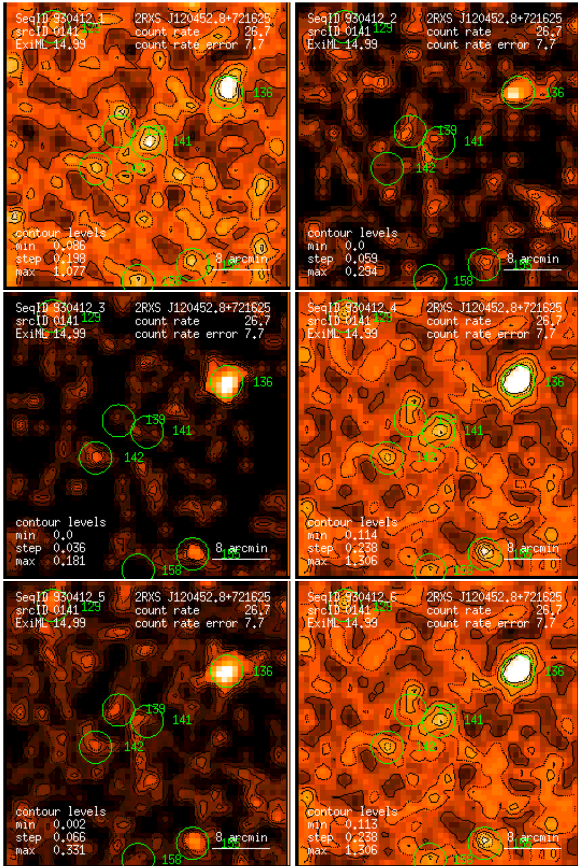
Figure 141: RASS 930412: detection 0141: band rate images, Gaussian filter: (1) PSPC channels 11 – 41, (2) 52 – 90, (3) 91 – 201, (4) 11 – 235, (5) 52 – 201, (6) 11 – 201. Broad band rates in counts/ks. Band rate contour levels in counts/ks/arcmin 2 .
