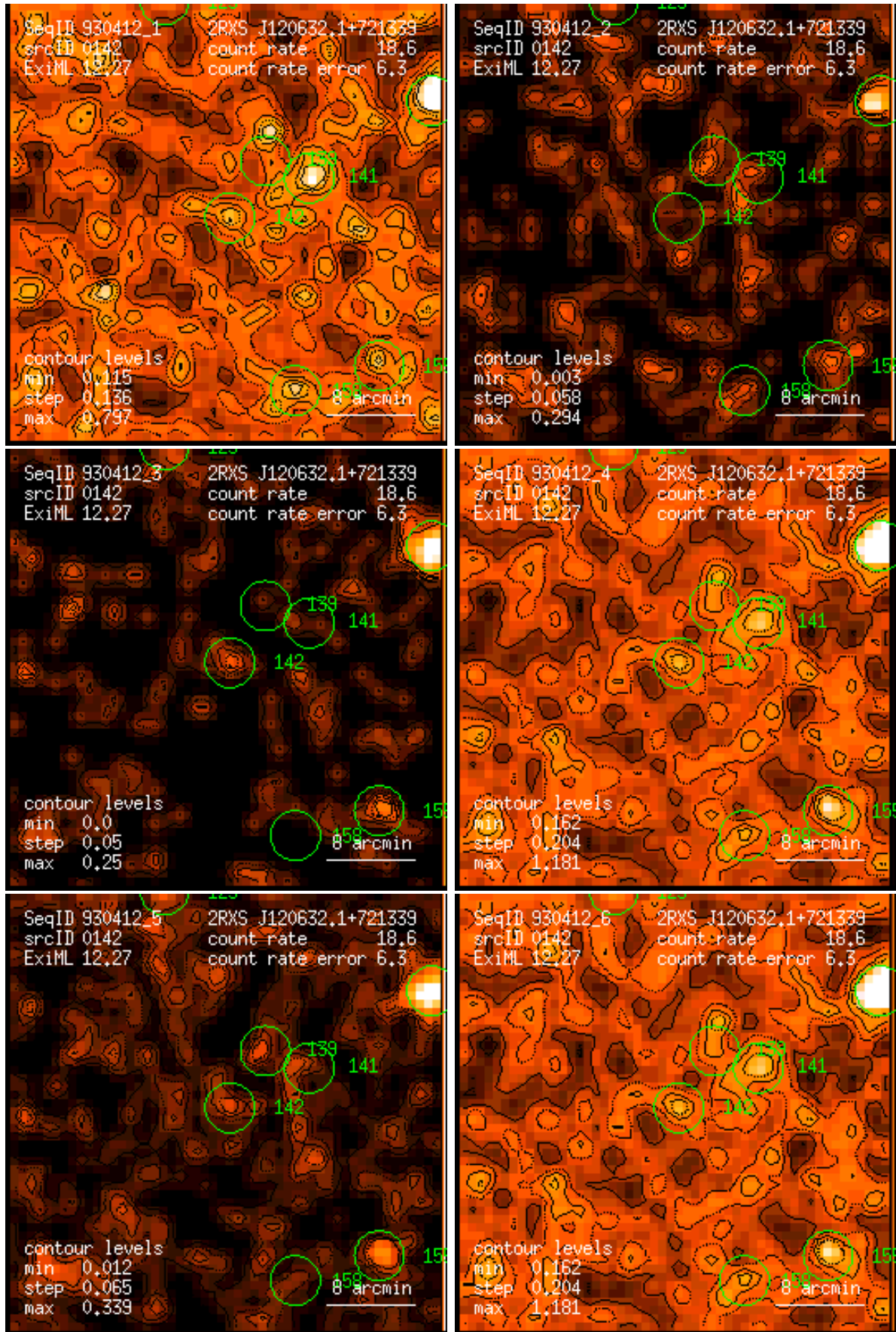
Figure 142: RASS 930412: detection 0142: band rate images, Gaussian filter: (1) PSPC channels 11 – 41, (2) 52 – 90, (3) 91 – 201, (4) 11 – 235, (5) 52 – 201, (6) 11 – 201. Broad band rates in counts/ks. Band rate contour levels in counts/ks/arcmin 2 .
