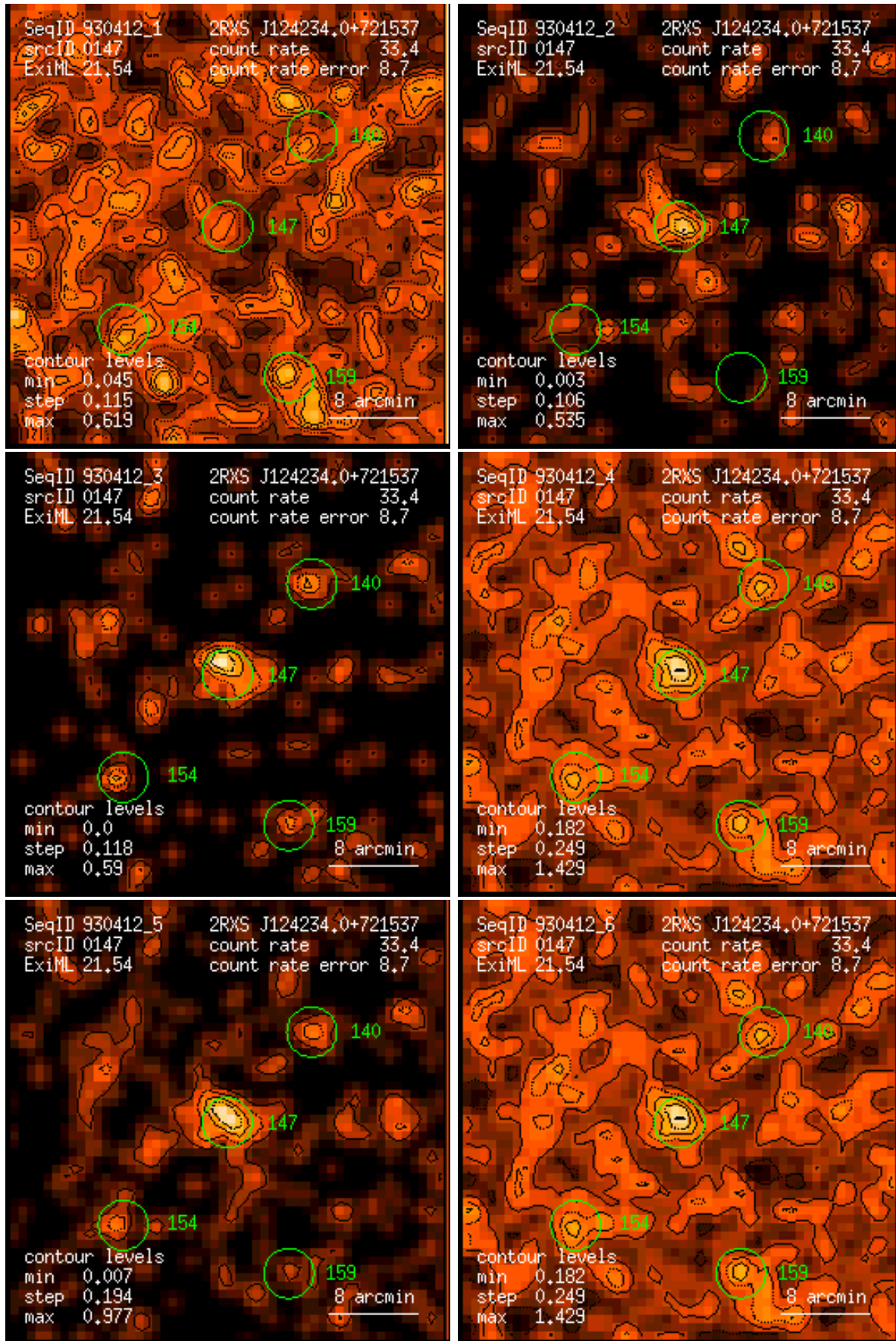
Figure 147: RASS 930412: detection 0147: band rate images, Gaussian filter: (1) PSPC channels 11 – 41, (2) 52 – 90, (3) 91 – 201, (4) 11 – 235, (5) 52 – 201, (6) 11 – 201. Broad band rates in counts/ks. Band rate contour levels in counts/ks/arcmin 2 .
