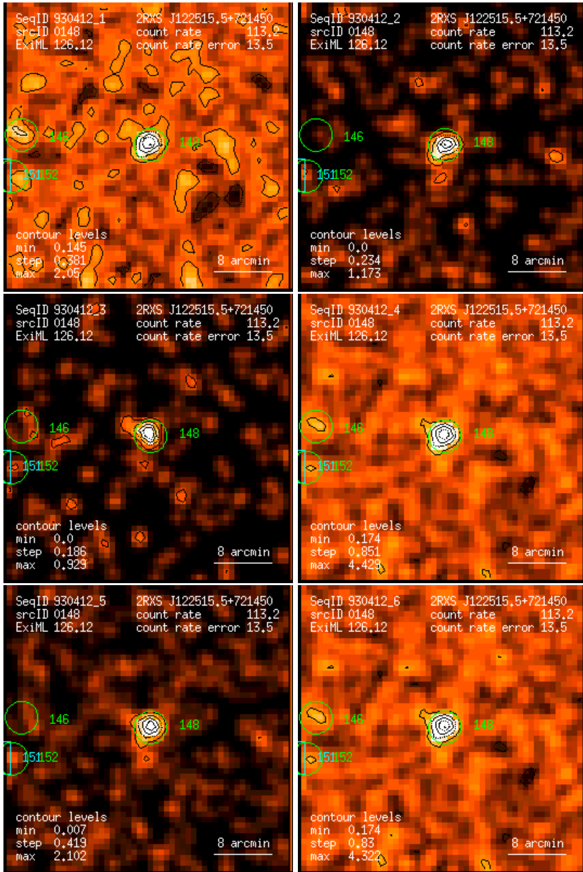
Figure 148: RASS 930412: detection 0148: band rate images, Gaussian filter: (1) PSPC channels 11 – 41, (2) 52 – 90, (3) 91 – 201, (4) 11 – 235, (5) 52 – 201, (6) 11 – 201. Broad band rates in counts/ks. Band rate contour levels in counts/ks/arcmin 2 .
