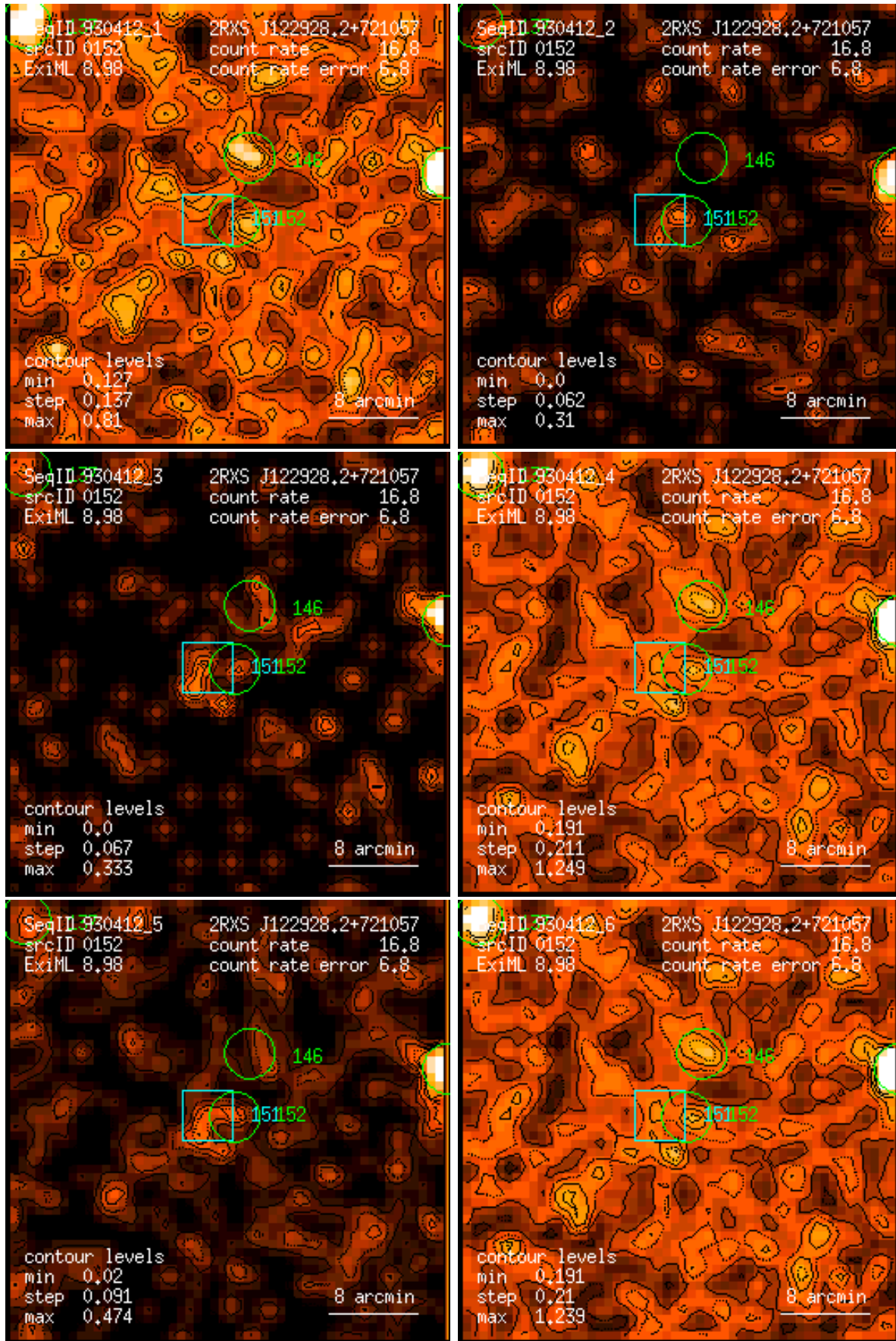
Figure 152: RASS 930412: detection 0152: band rate images, Gaussian filter: (1) PSPC channels 11 – 41, (2) 52 – 90, (3) 91 – 201, (4) 11 – 235, (5) 52 – 201, (6) 11 – 201. Broad band rates in counts/ks. Band rate contour levels in counts/ks/arcmin 2 .
