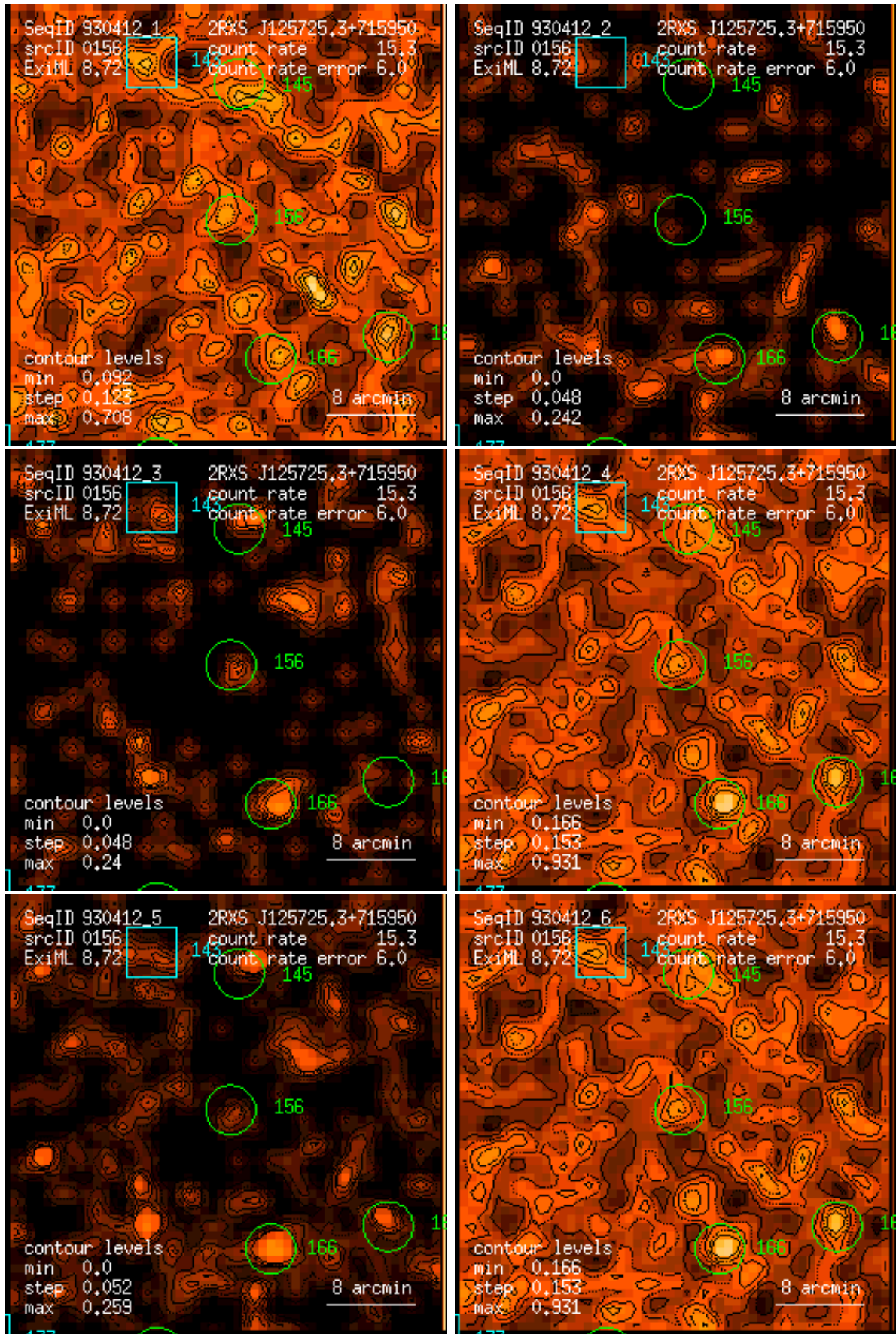
Figure 156: RASS 930412: detection 0156: band rate images, Gaussian filter: (1) PSPC channels 11 – 41, (2) 52 – 90, (3) 91 – 201, (4) 11 – 235, (5) 52 – 201, (6) 11 – 201. Broad band rates in counts/ks. Band rate contour levels in counts/ks/arcmin 2 .
