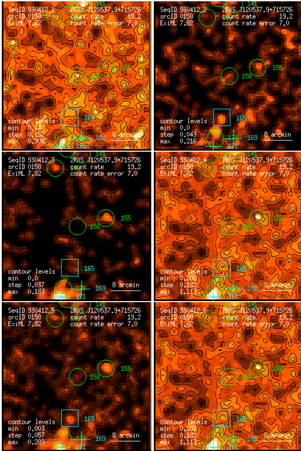
Figure 158: RASS 930412: detection 0158: band rate images, Gaussian filter: (1) PSPC channels 11 – 41, (2) 52 – 90, (3) 91 – 201, (4) 11 – 235, (5) 52 – 201, (6) 11 – 201. Broad band rates in counts/ks. Band rate contour levels in counts/ks/arcmin 2 .
