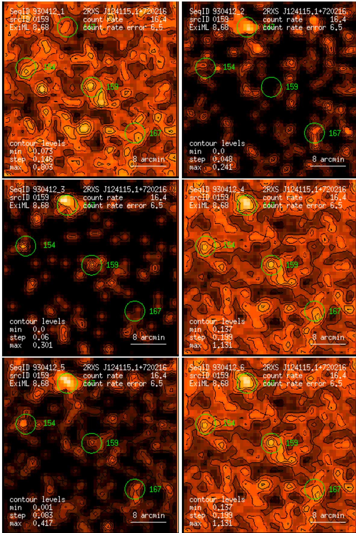
Figure 159: RASS 930412: detection 0159: band rate images, Gaussian filter: (1) PSPC channels 11 – 41, (2) 52 – 90, (3) 91 – 201, (4) 11 – 235, (5) 52 – 201, (6) 11 – 201. Broad band rates in counts/ks. Band rate contour levels in counts/ks/arcmin 2 .
