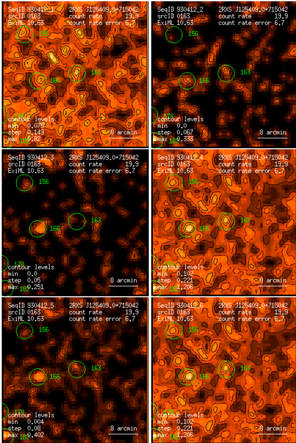
Figure 163: RASS 930412: detection 0163: band rate images, Gaussian filter: (1) PSPC channels 11 – 41, (2) 52 – 90, (3) 91 – 201, (4) 11 – 235, (5) 52 – 201, (6) 11 – 201. Broad band rates in counts/ks. Band rate contour levels in counts/ks/arcmin 2 .
