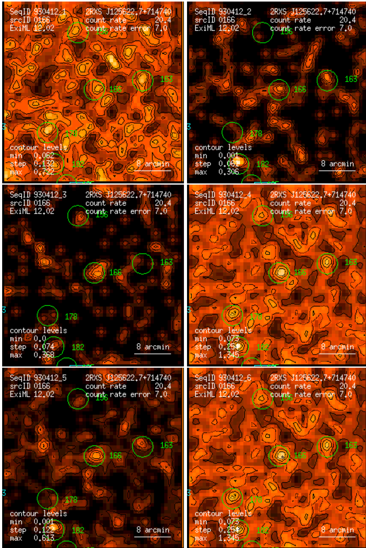
Figure 166: RASS 930412: detection 0166: band rate images, Gaussian filter: (1) PSPC channels 11 – 41, (2) 52 – 90, (3) 91 – 201, (4) 11 – 235, (5) 52 – 201, (6) 11 – 201. Broad band rates in counts/ks. Band rate contour levels in counts/ks/arcmin 2 .
