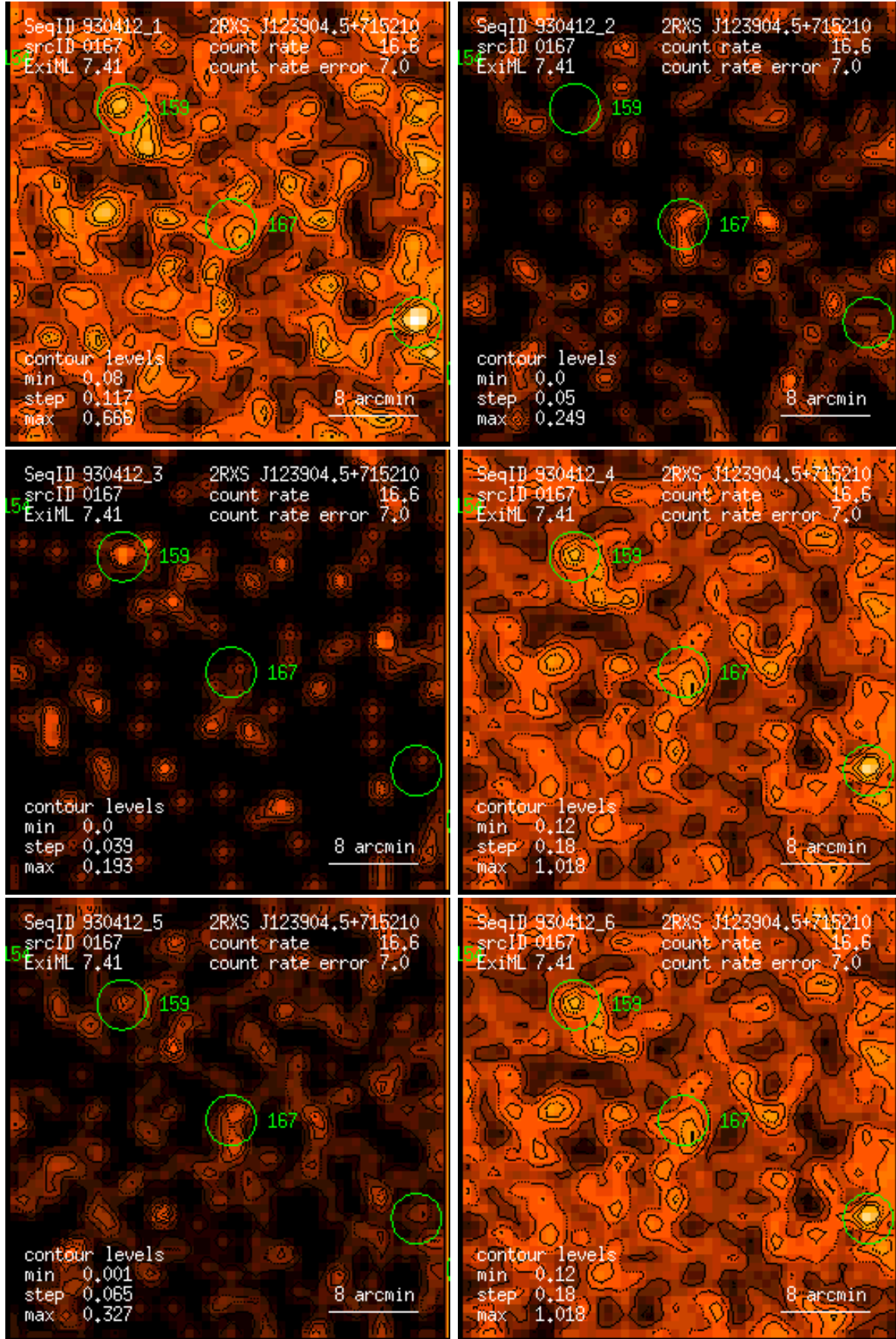
Figure 167: RASS 930412: detection 0167: band rate images, Gaussian filter: (1) PSPC channels 11 – 41, (2) 52 – 90, (3) 91 – 201, (4) 11 – 235, (5) 52 – 201, (6) 11 – 201. Broad band rates in counts/ks. Band rate contour levels in counts/ks/arcmin 2 .
