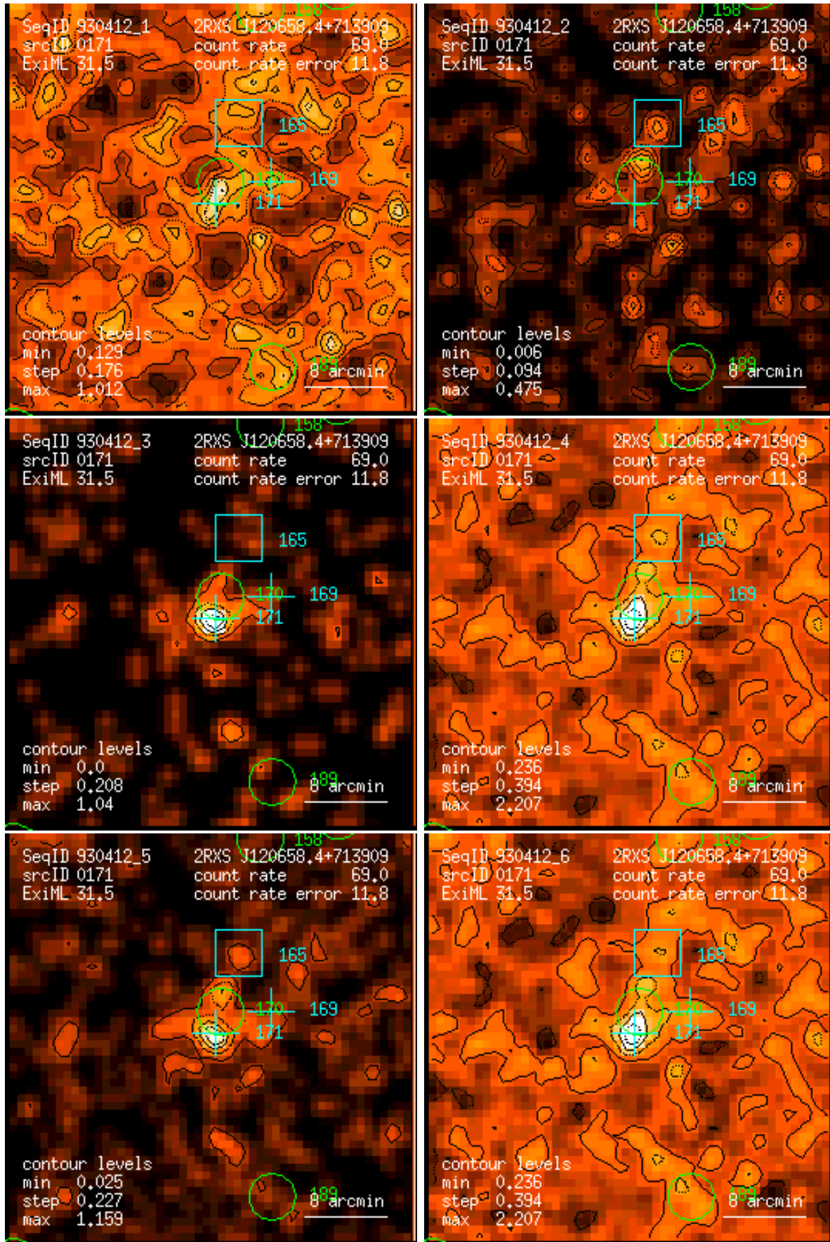
Figure 171: RASS 930412: detection 0171: band rate images, Gaussian filter: (1) PSPC channels 11 – 41, (2) 52 – 90, (3) 91 – 201, (4) 11 – 235, (5) 52 – 201, (6) 11 – 201. Broad band rates in counts/ks. Band rate contour levels in counts/ks/arcmin 2 .
