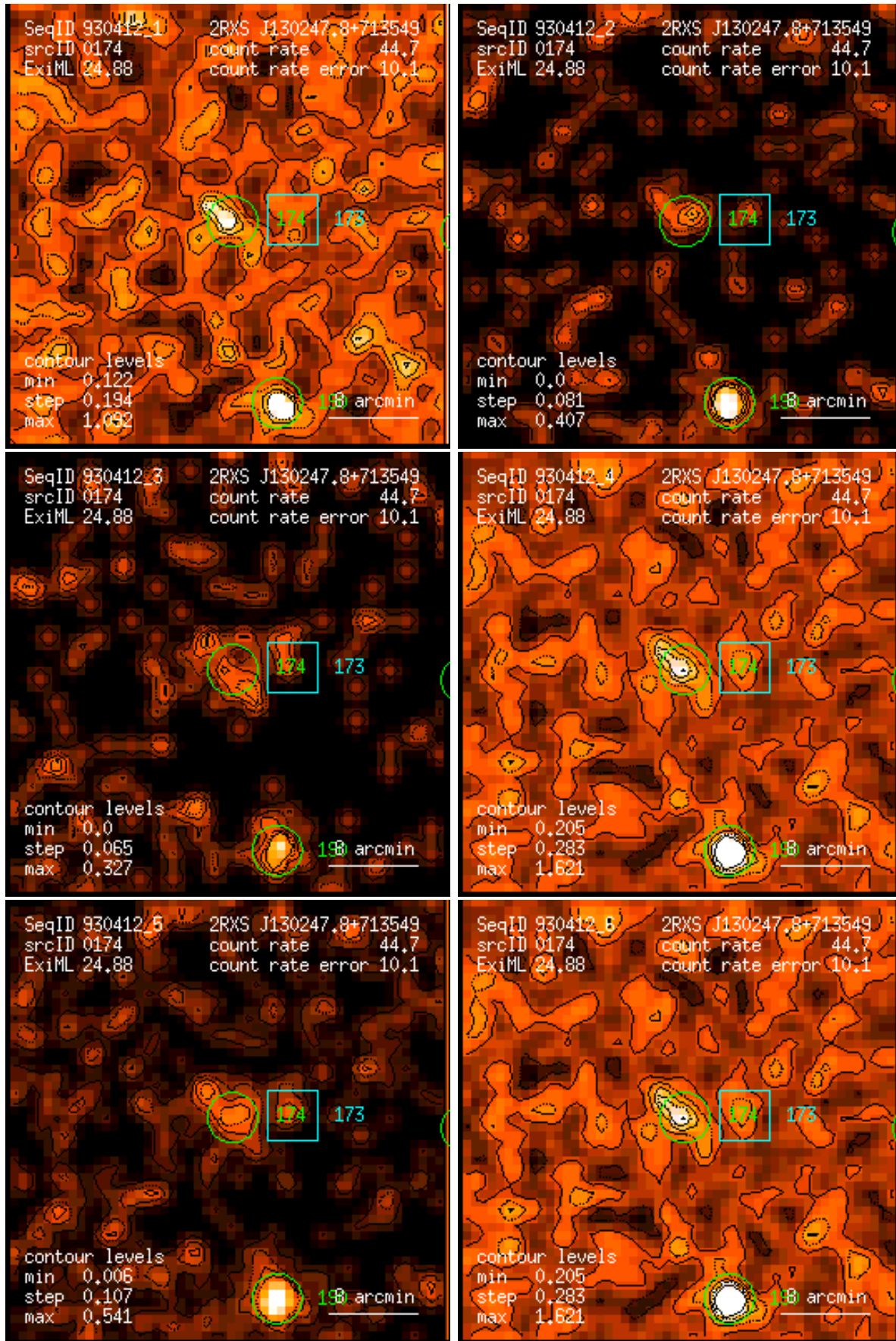
Figure 174: RASS 930412: detection 0174: band rate images, Gaussian filter: (1) PSPC channels 11 – 41, (2) 52 – 90, (3) 91 – 201, (4) 11 – 235, (5) 52 – 201, (6) 11 – 201. Broad band rates in counts/ks. Band rate contour levels in counts/ks/arcmin 2 .
