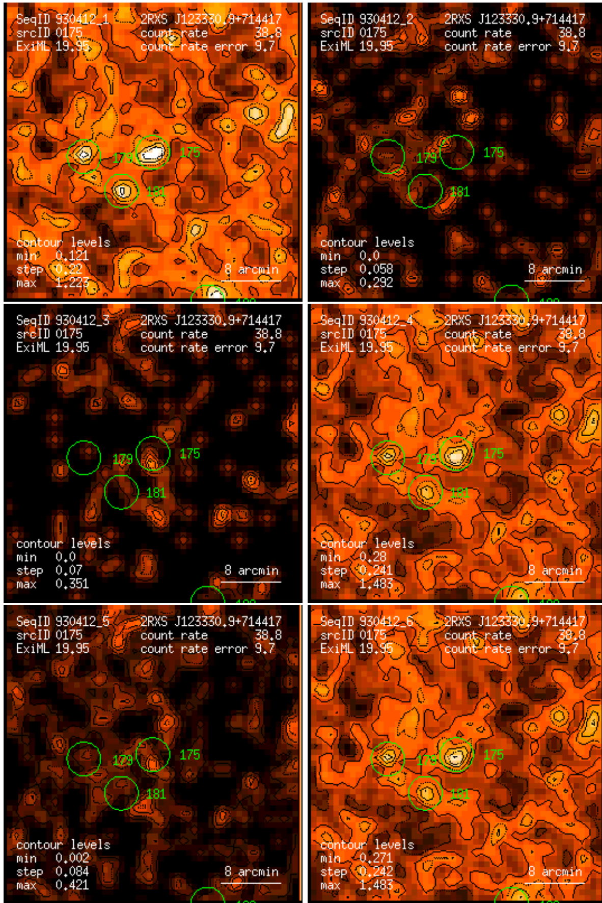
Figure 175: RASS 930412: detection 0175: band rate images, Gaussian filter: (1) PSPC channels 11 – 41, (2) 52 – 90, (3) 91 – 201, (4) 11 – 235, (5) 52 – 201, (6) 11 – 201. Broad band rates in counts/ks. Band rate contour levels in counts/ks/arcmin 2 .
