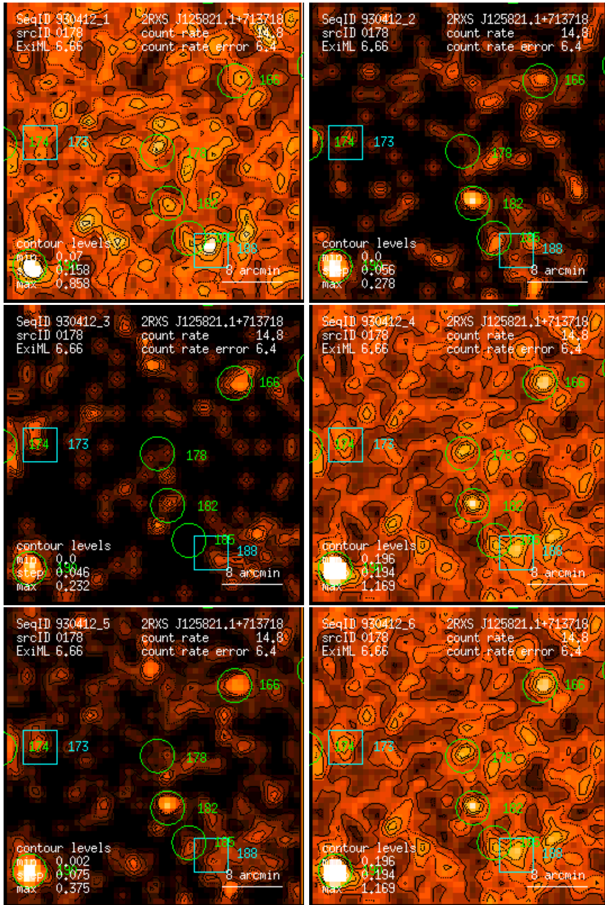
Figure 178: RASS 930412: detection 0178: band rate images, Gaussian filter: (1) PSPC channels 11 – 41, (2) 52 – 90, (3) 91 – 201, (4) 11 – 235, (5) 52 – 201, (6) 11 – 201. Broad band rates in counts/ks. Band rate contour levels in counts/ks/arcmin 2 .
