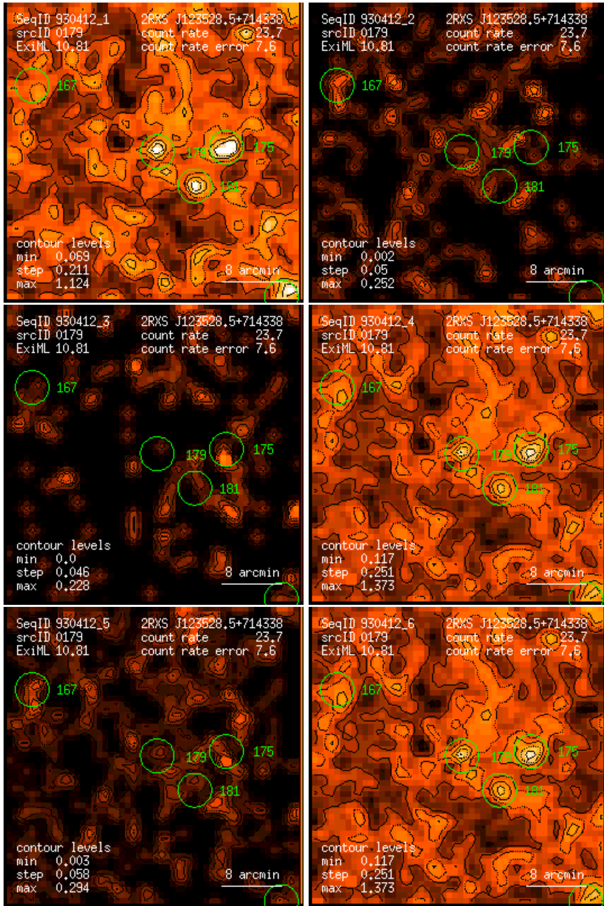
Figure 179: RASS 930412: detection 0179: band rate images, Gaussian filter: (1) PSPC channels 11 – 41, (2) 52 – 90, (3) 91 – 201, (4) 11 – 235, (5) 52 – 201, (6) 11 – 201. Broad band rates in counts/ks. Band rate contour levels in counts/ks/arcmin 2 .
