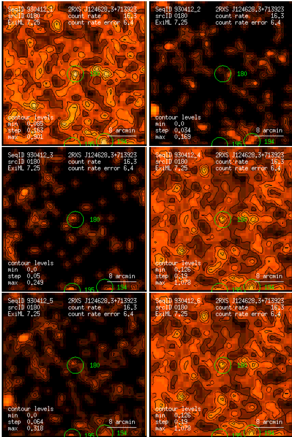
Figure 180: RASS 930412: detection 0180: band rate images, Gaussian filter: (1) PSPC channels 11 – 41, (2) 52 – 90, (3) 91 – 201, (4) 11 – 235, (5) 52 – 201, (6) 11 – 201. Broad band rates in counts/ks. Band rate contour levels in counts/ks/arcmin 2 .
