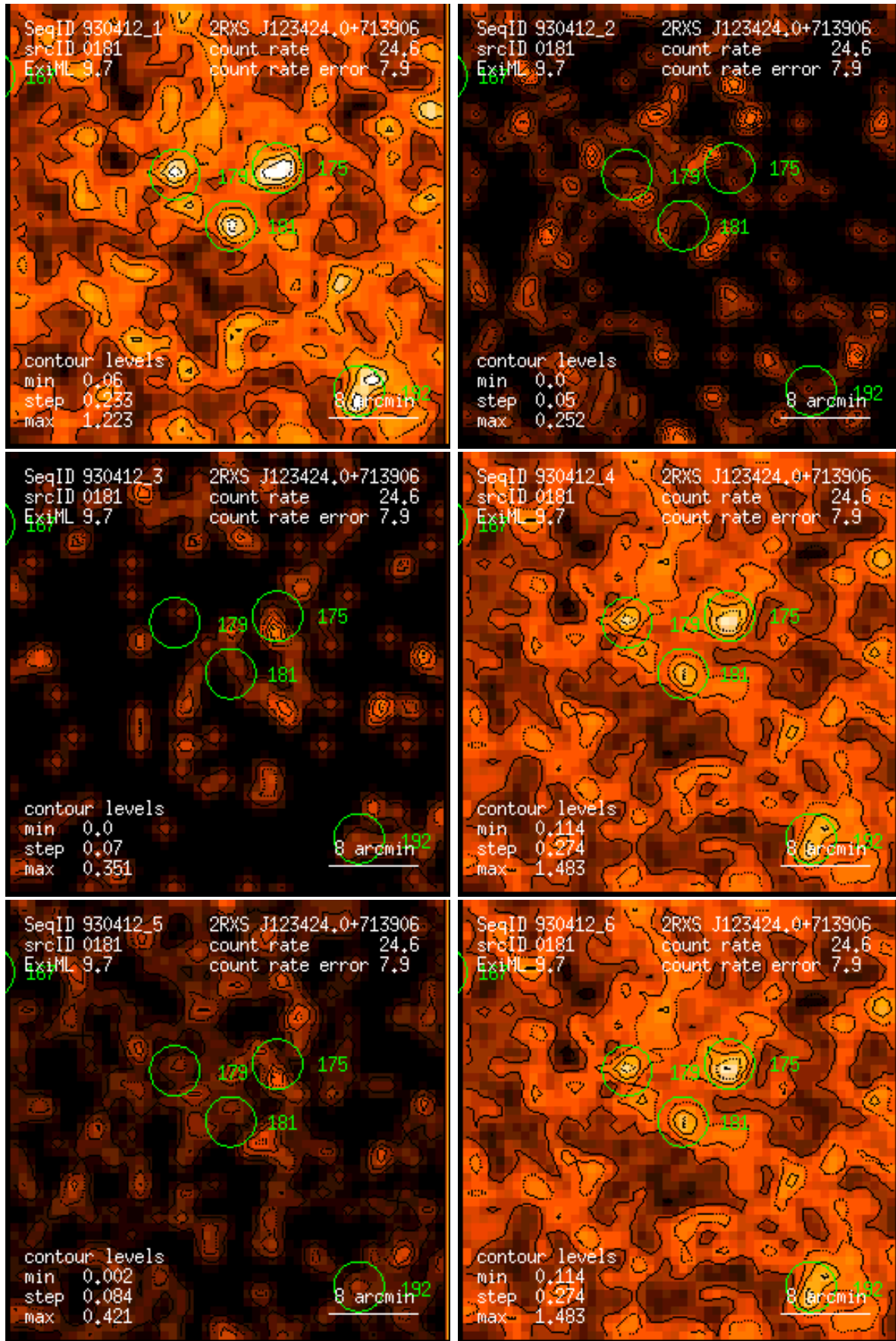
Figure 181: RASS 930412: detection 0181: band rate images, Gaussian filter: (1) PSPC channels 11 – 41, (2) 52 – 90, (3) 91 – 201, (4) 11 – 235, (5) 52 – 201, (6) 11 – 201. Broad band rates in counts/ks. Band rate contour levels in counts/ks/arcmin 2 .
