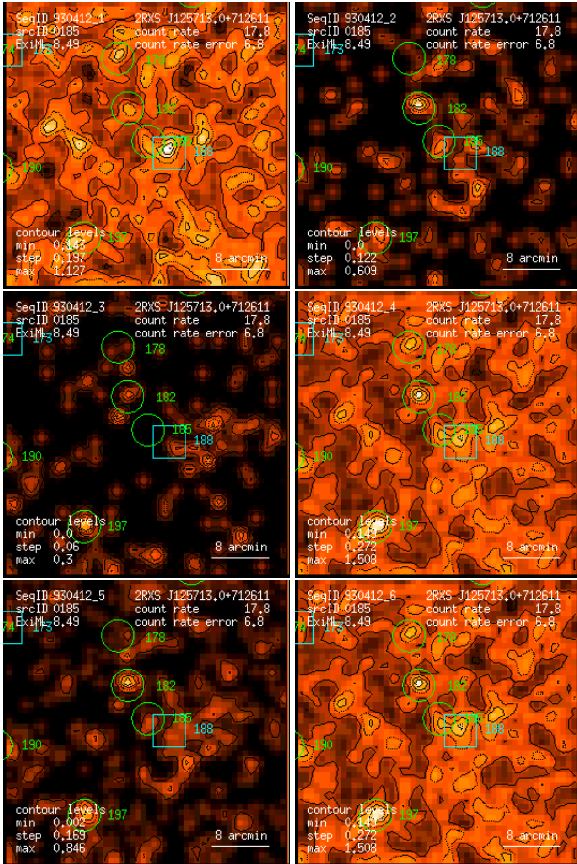
Figure 185: RASS 930412: detection 0185: band rate images, Gaussian filter: (1) PSPC channels 11 – 41, (2) 52 – 90, (3) 91 – 201, (4) 11 – 235, (5) 52 – 201, (6) 11 – 201. Broad band rates in counts/ks. Band rate contour levels in counts/ks/arcmin 2 .
