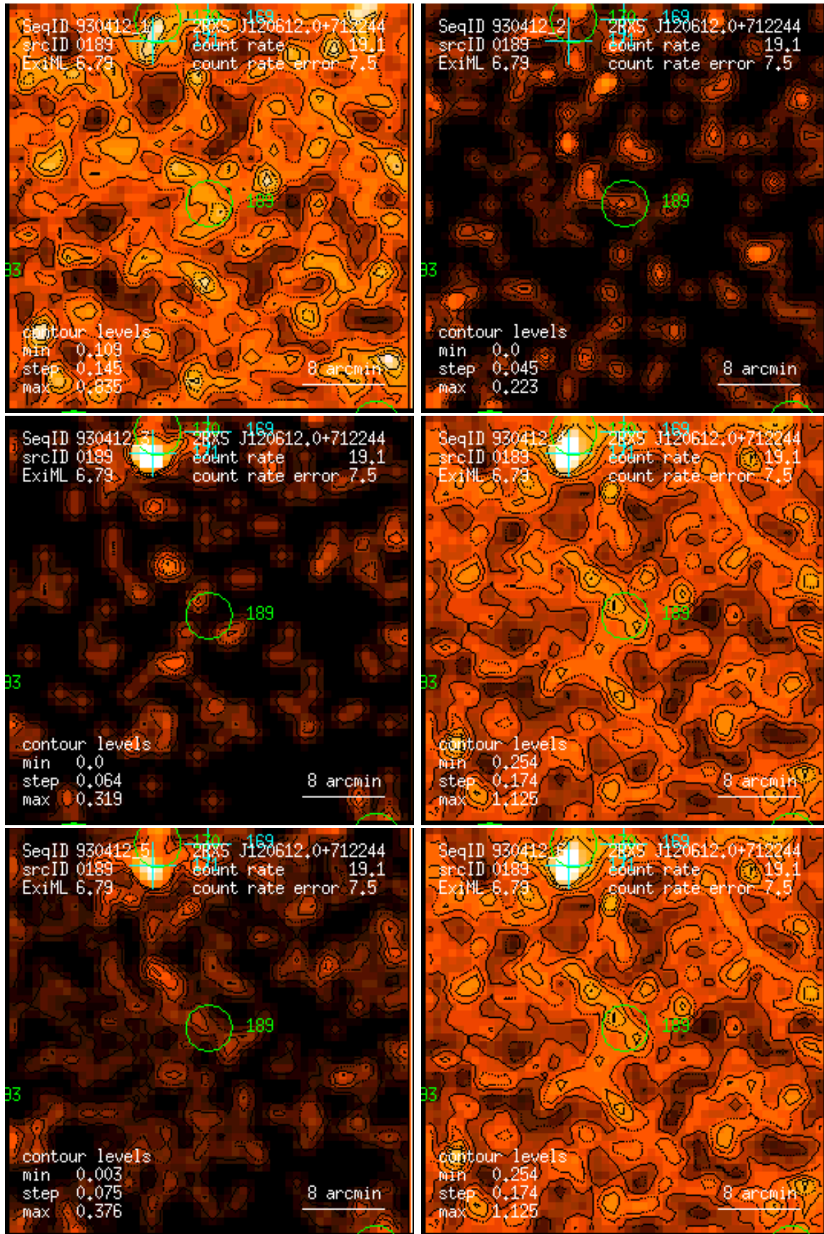
Figure 189: RASS 930412: detection 0189: band rate images, Gaussian filter: (1) PSPC channels 11 – 41, (2) 52 – 90, (3) 91 – 201, (4) 11 – 235, (5) 52 – 201, (6) 11 – 201. Broad band rates in counts/ks. Band rate contour levels in counts/ks/arcmin 2 .
