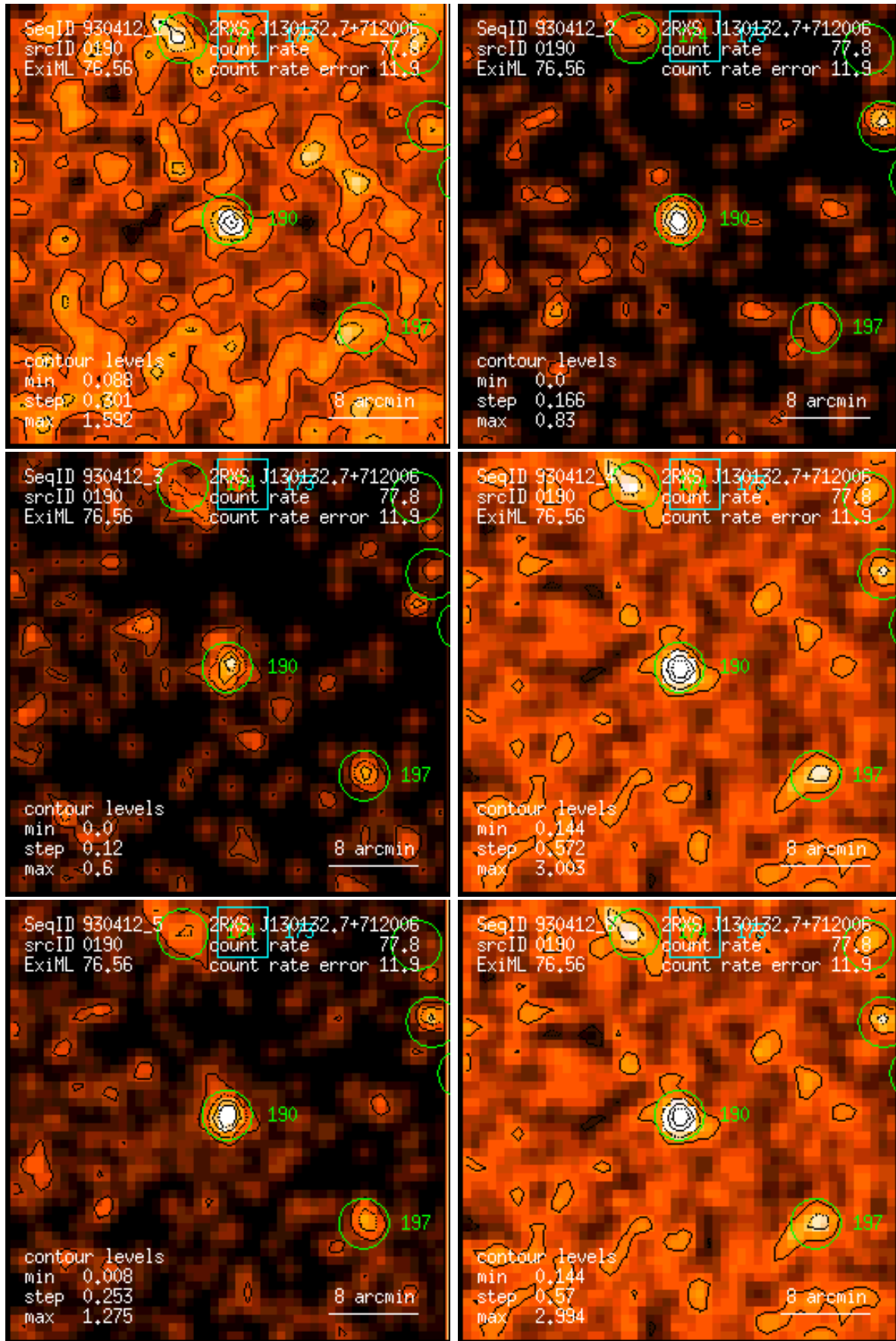
Figure 190: RASS 930412: detection 0190: band rate images, Gaussian filter: (1) PSPC channels 11 – 41, (2) 52 – 90, (3) 91 – 201, (4) 11 – 235, (5) 52 – 201, (6) 11 – 201. Broad band rates in counts/ks. Band rate contour levels in counts/ks/arcmin 2 .
