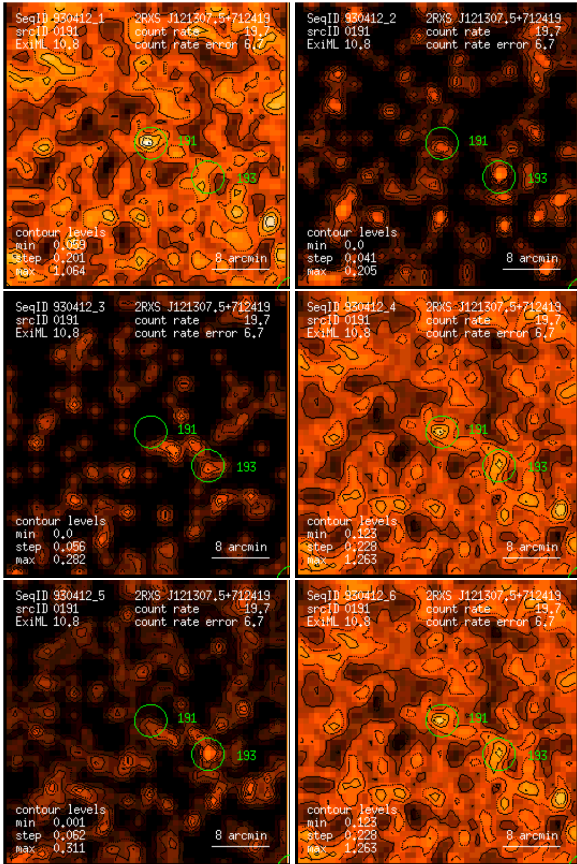
Figure 191: RASS 930412: detection 0191: band rate images, Gaussian filter: (1) PSPC channels 11 – 41, (2) 52 – 90, (3) 91 – 201, (4) 11 – 235, (5) 52 – 201, (6) 11 – 201. Broad band rates in counts/ks. Band rate contour levels in counts/ks/arcmin 2 .
